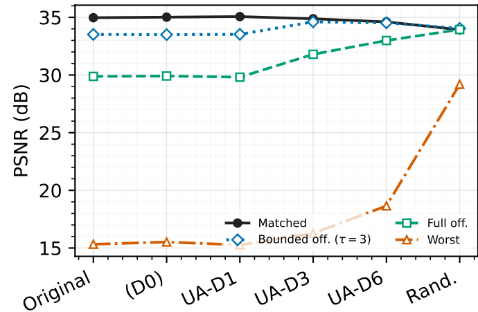
(a) Robustness--fidelity trade-off
