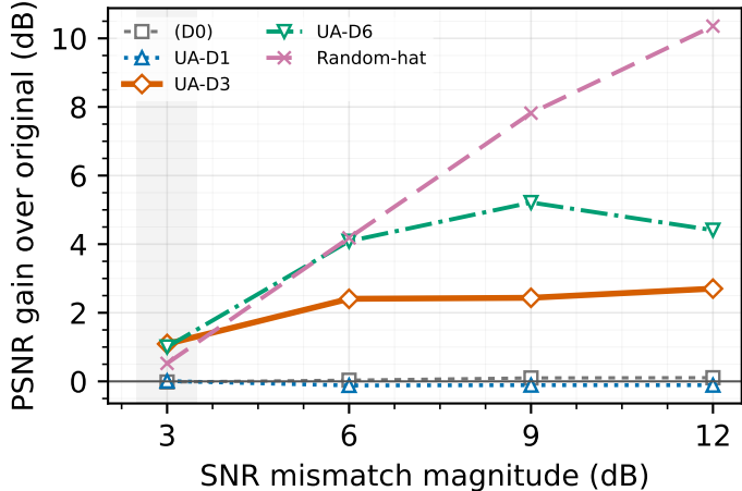
(b) Robustness by mismatch magnitude
