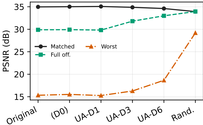
Robustness--fidelity trade-off
