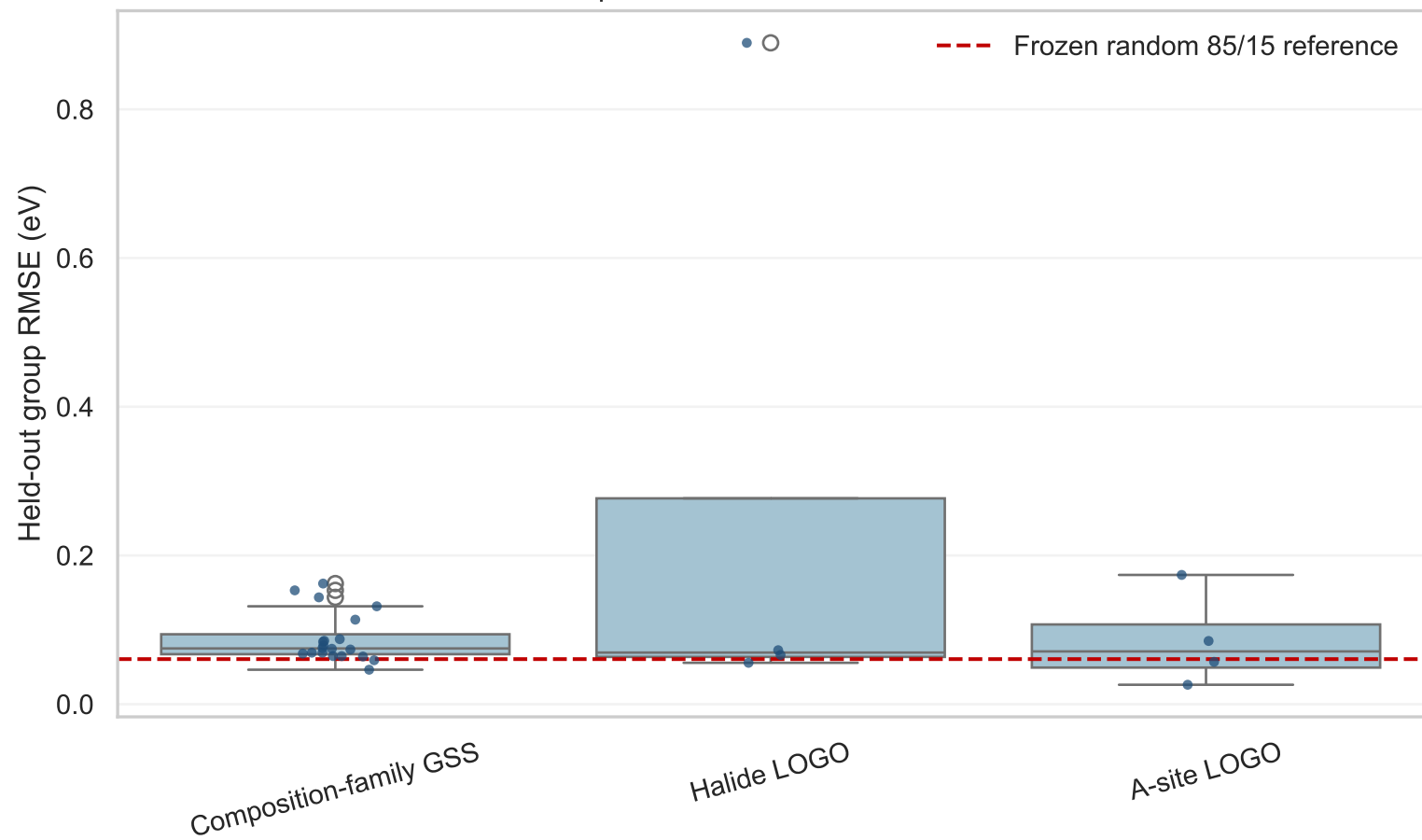
Group-aware test RMSE distribution
