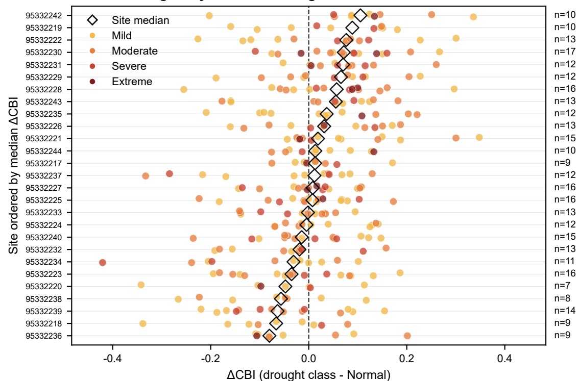
D Site heterogeneity across all drought classes
