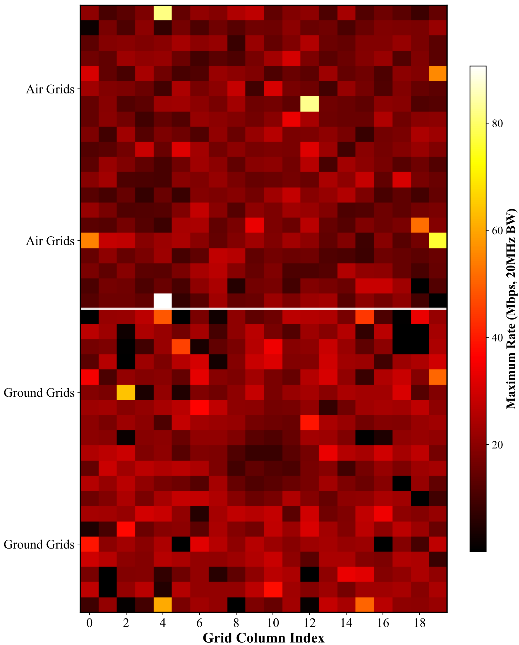
Grid Performance Heatmap: Maximum Theoretical Rate
