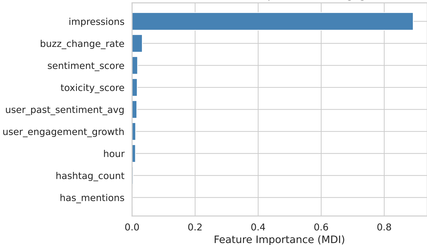
Random Forest Feature Importance for Engagement Rate
