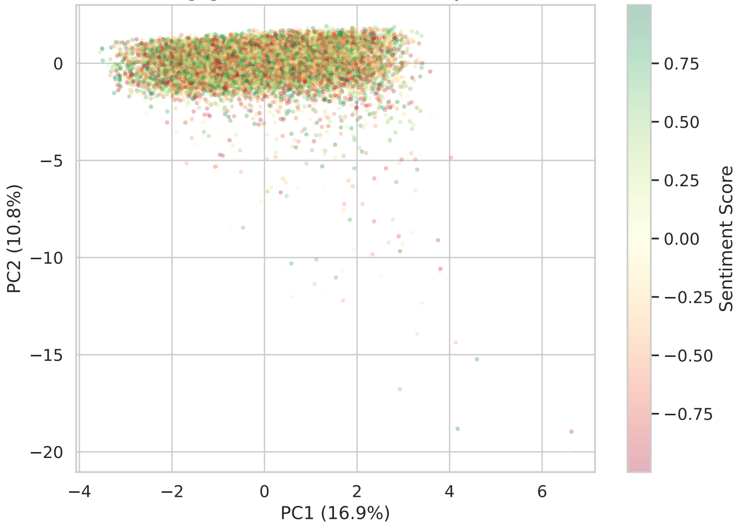
PCA of Engagement Features (colored by Sentiment)
