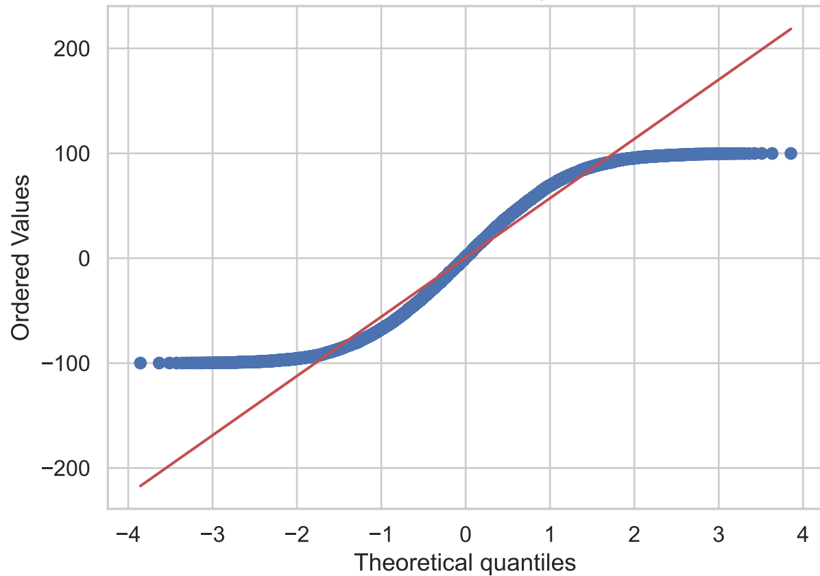
Q-Q Plot: Buzz Change Rate
