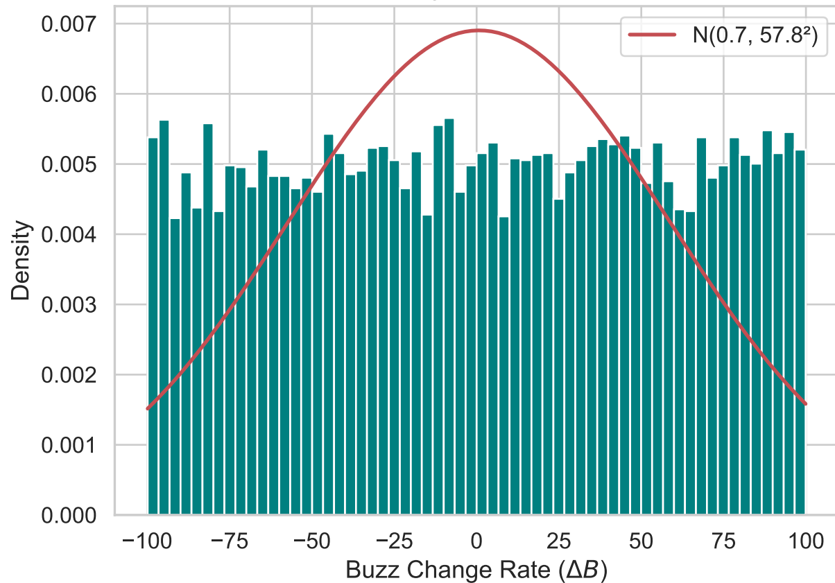
Buzz Change Rate Distribution
