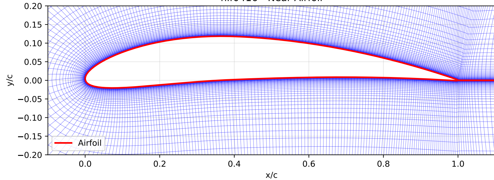
nlf0416 - Near Airfoil
