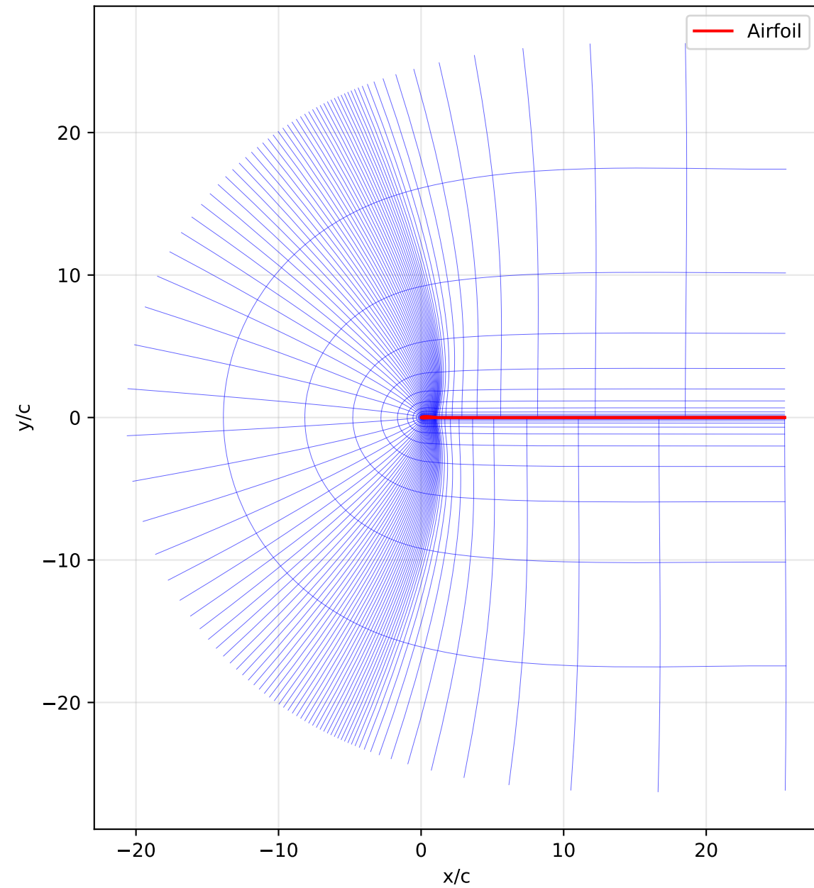
naca2412 - Full Domain
