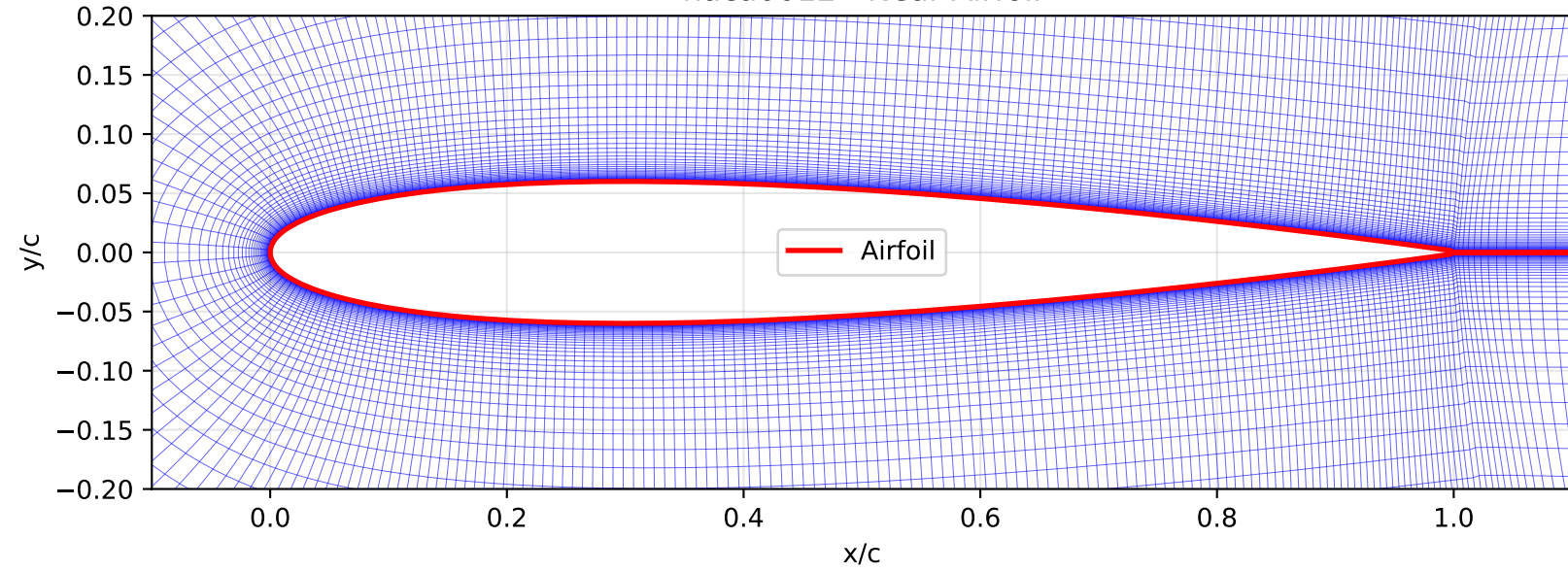
naca0012 - Near Airfoil
