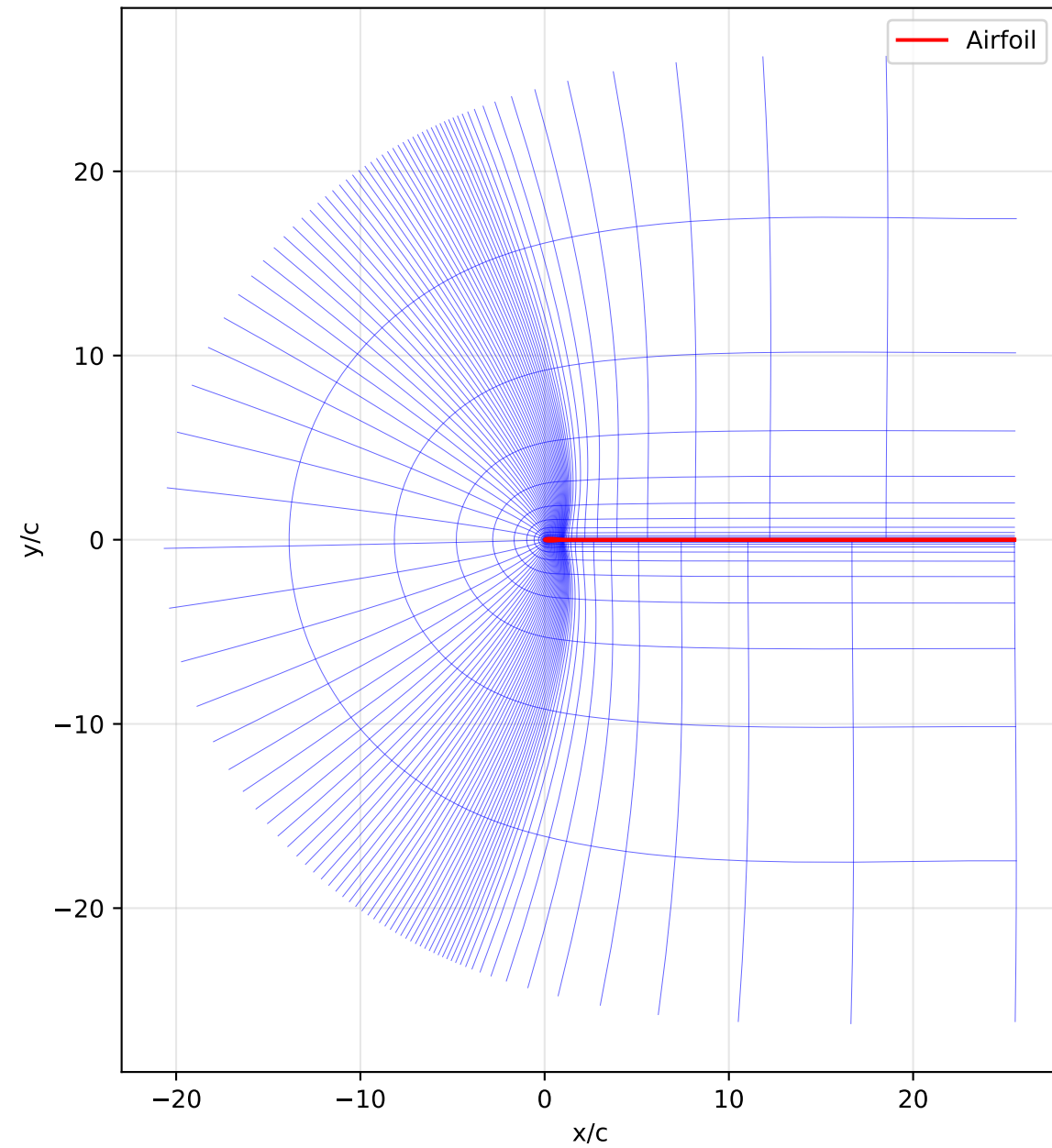
naca0012 - Full Domain
