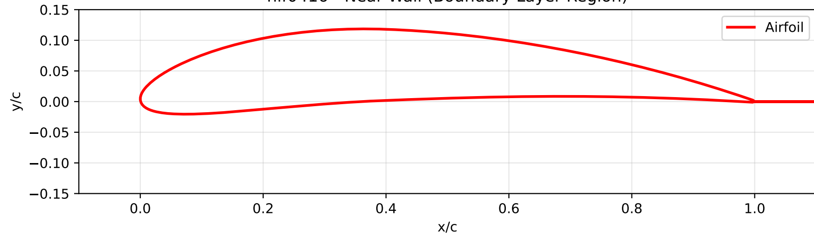
nlf0416 - Near Wall (Boundary Layer Region)
