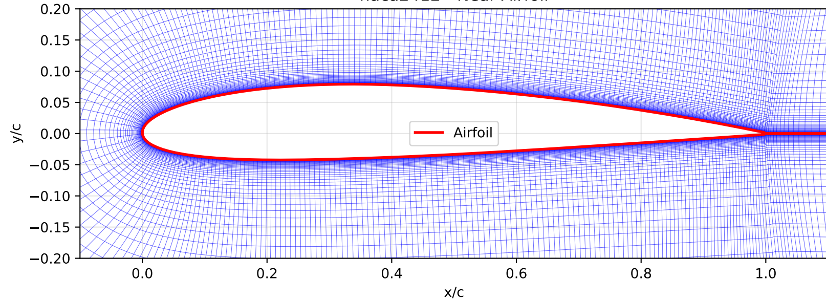
naca2412 - Near Airfoil
