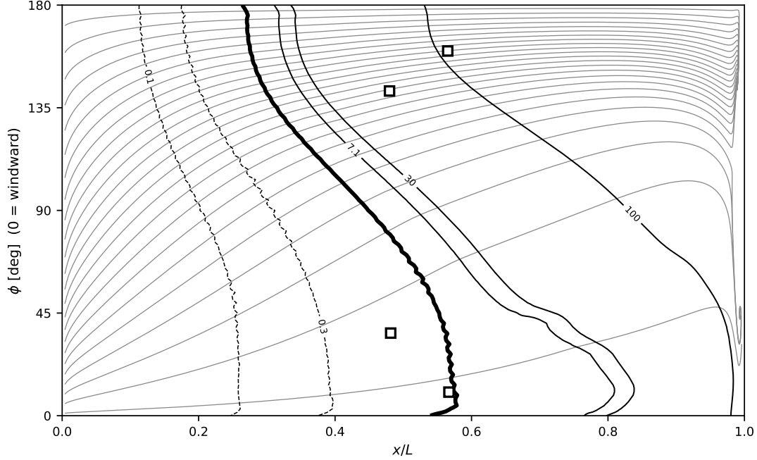
Fig. 27 \alpha = 5^\circ , Re_L = 6.49 \times 10^6 .
