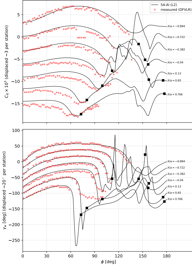
Fig. 31 As Fig. 30, at \alpha = 29.7^\circ (presentation of Stock's Fig. 5); measured chains truncated in the leeward tangle where printed chain identity is unrecoverable.
