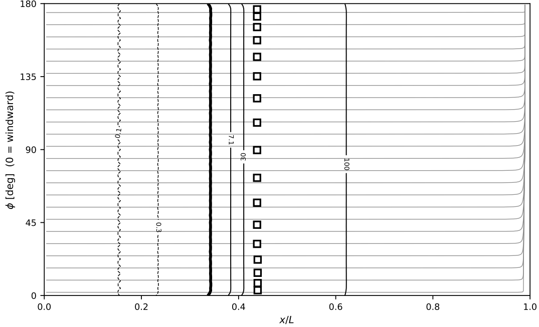
Fig. 24 Surface unrolled into (x/L, \phi) , \phi=0 the windward symmetry line, at the measured-seed condition. Grey: skin-friction lines integrated from the wall shear vector itself—the oil-flow analogue, and not the inviscid streamlines of Stock Figs. 14–17—whose convergence marks separation. Black: the \max_n \chi family on a wall-normal segment shot from each surface point, sub-unity decades dashed, \chi = 1 heavy, \chi = c_{v1} and above solid. White-filled squares: the measured DFVLR transition points. Zero incidence, Re_L = 7.2 \times 10^6 : both families are functions of x/L alone, as the axisymmetric flow requires.
