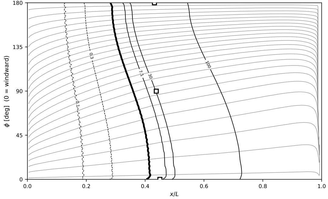
Fig. 25 \alpha = 2.5^\circ , Re_L = 7.2 \times 10^6 .
