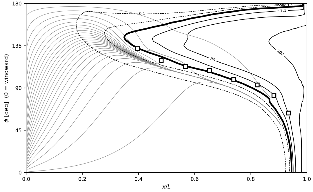
Fig. 32 \alpha = 10^\circ , Re_L = 1.52 \times 10^6 .
