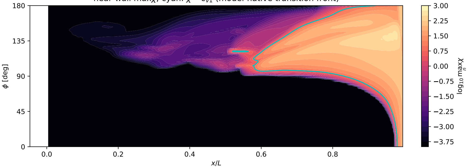
near-wall \max \chi ; cyan: \chi = c_{v1} (model-native transition front)
