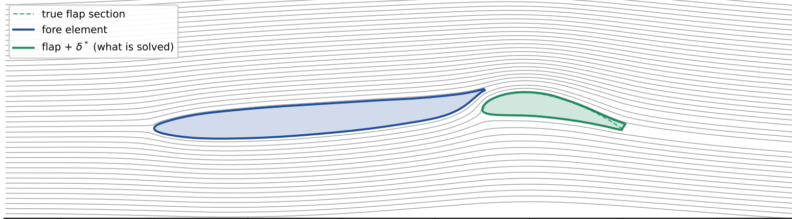
Adopted two-element geometry, inviscid: \alpha = -1.0^\circ , C_L = 0.412
