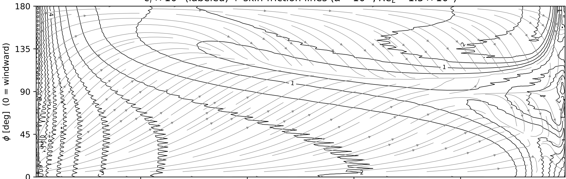
wall-shear direction \gamma_w [deg] from local meridian (positive toward leeward; dashed negative; bold: \gamma_w = 0 )
