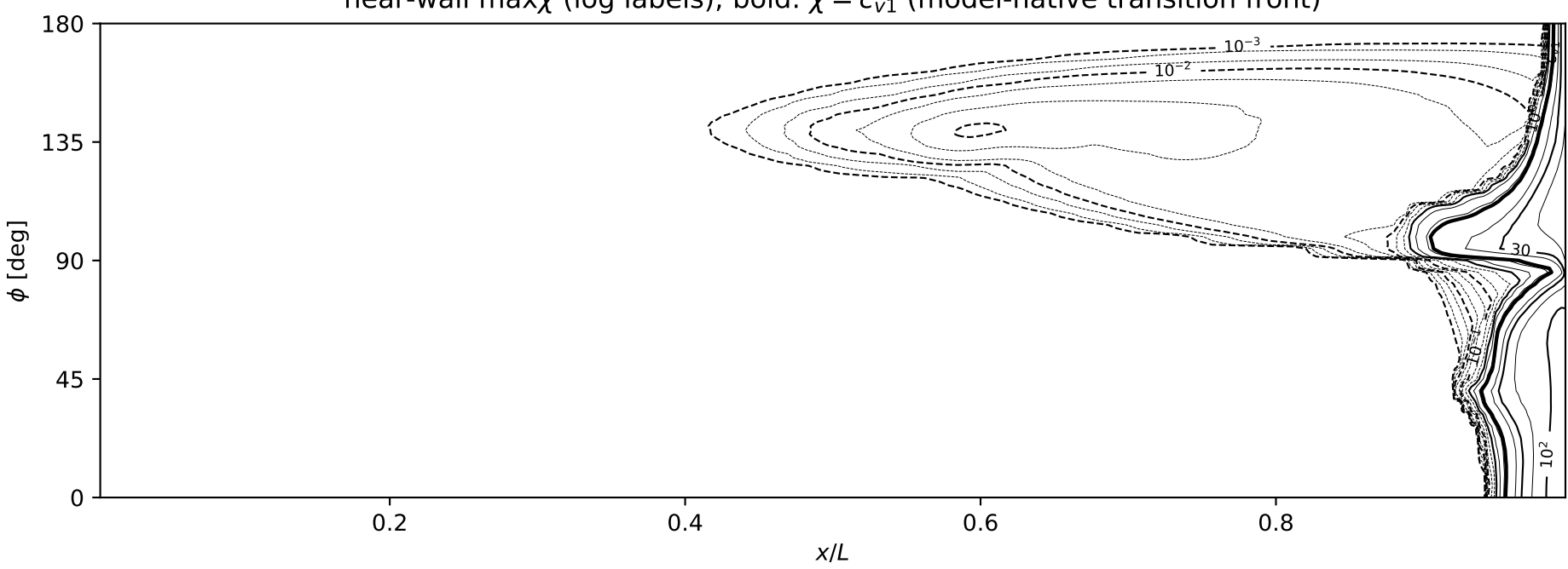
near-wall \max \chi (log labels); bold: \chi = c_{v1} (model-native transition front)
