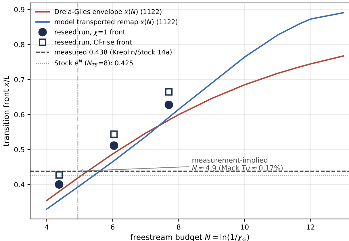
6:1 spheroid, \alpha = 0 , Re_L = 7.2 \times 10^6 : front vs freestream seed
