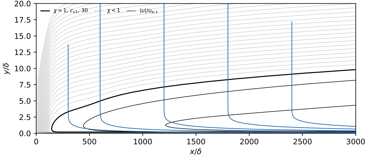
Figure 5: Attachment-anchored turbulent branch, L = 3000 ( Re_r = 9 \times 10^6 ), \max \chi = 76 . Standard SA, frozen Hiemenz, \chi_\infty = 0 . \chi contours dashed per decade for \chi < 1 ( 10^{-24} – 10^{-1} ; the zero freestream leaves no floor, so \chi decays smoothly over decades), solid at 1, c_{v1} , 30; velocity magnitude |u|/u_{e,L} (blue, normalized by the x=L edge speed) at 0.1, 0.2, 0.4, 0.6, 0.8. Branch data in Table 1.
