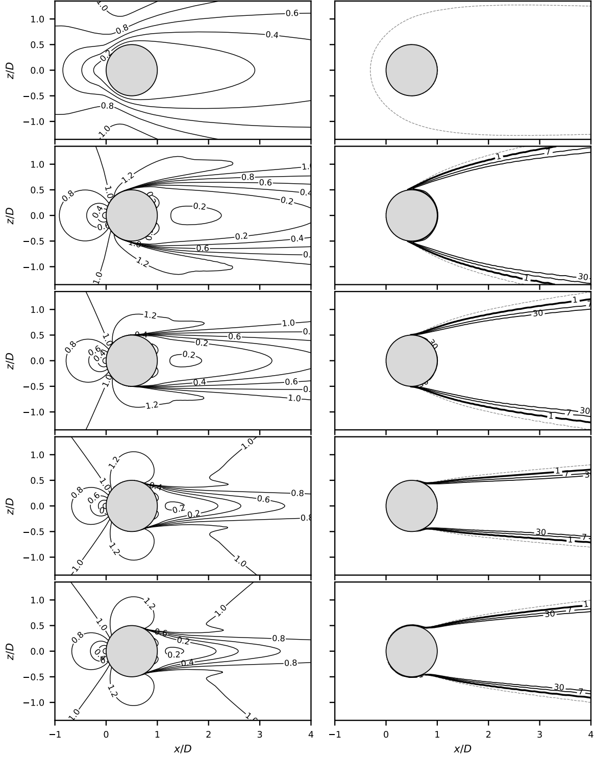
Figure 22: Drag-crisis fields, Re_D = 10, 10^5, 5 \times 10^5, 2 \times 10^6, 10^9 (rows, up-ladder Tu = 0.2\% ); columns |\mathbf{u}|/U_\infty and \chi (dashed \chi < 1 , solid \chi = 1, c_{v1}, 30 ). C_d = 2.80, 0.84, 0.62, 0.22, 0.21 .
