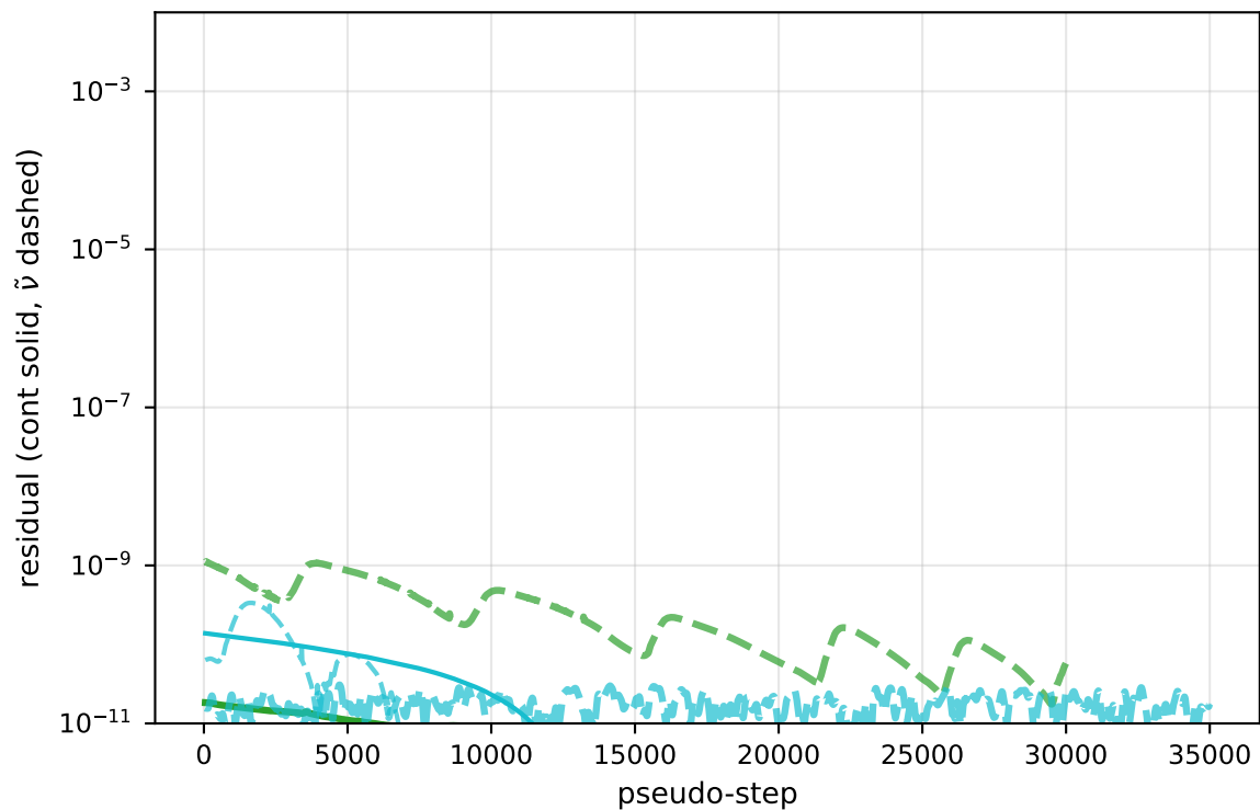
\alpha=7^\circ : residuals
