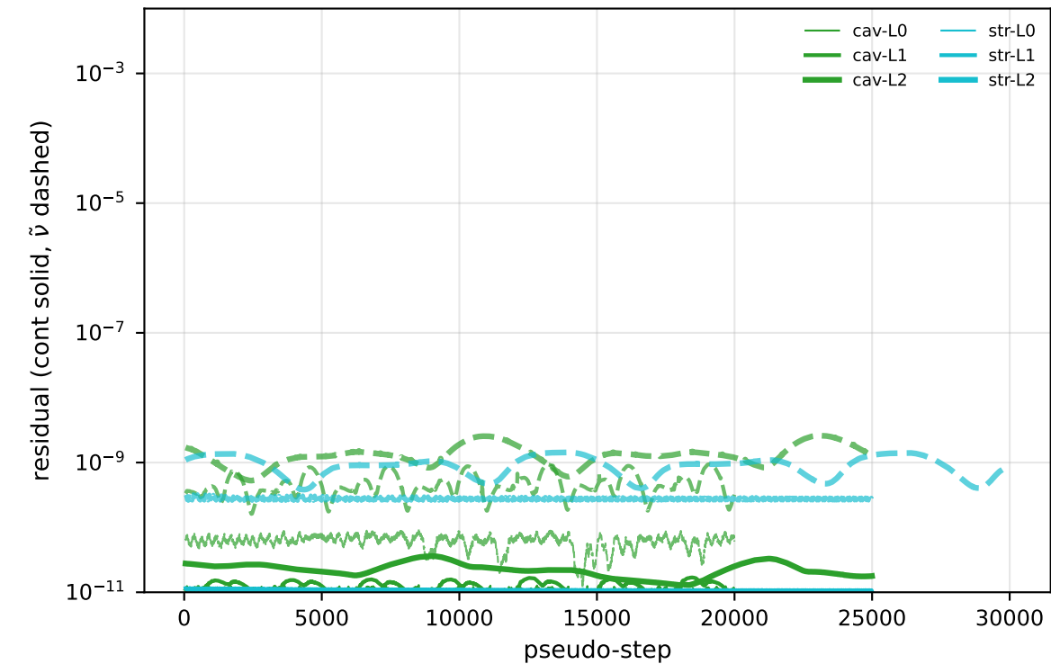
\alpha=2^\circ : residuals
