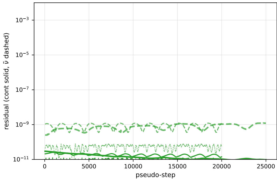
\alpha=2^\circ : residuals
