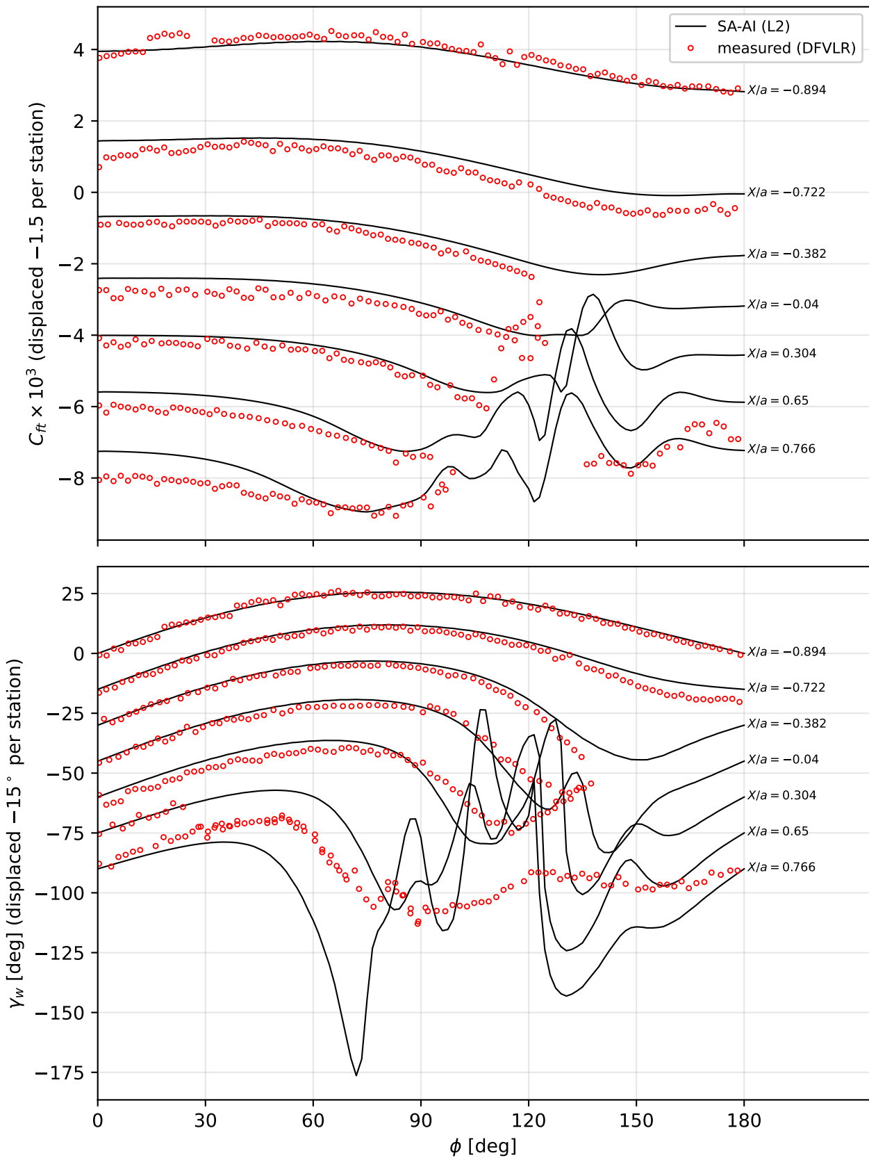
\alpha = 10^\circ , Re_L = 1.5 \times 10^6 (L2): wall shear at the DFVLR hot-film stations
