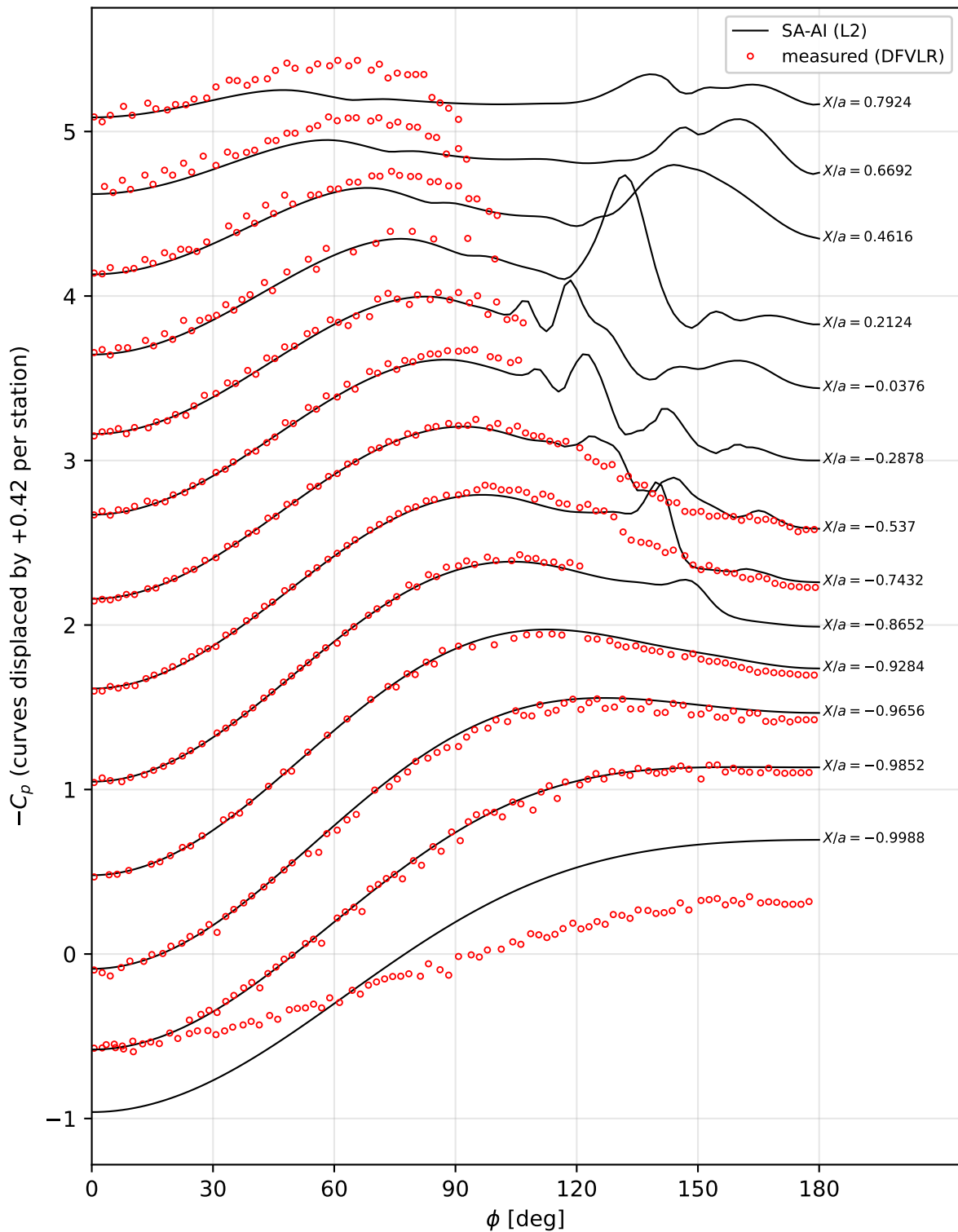
\alpha = 29.7^\circ , Re_L = 1.5 \times 10^6 (L2): C_p at the DFVLR pressure stations
