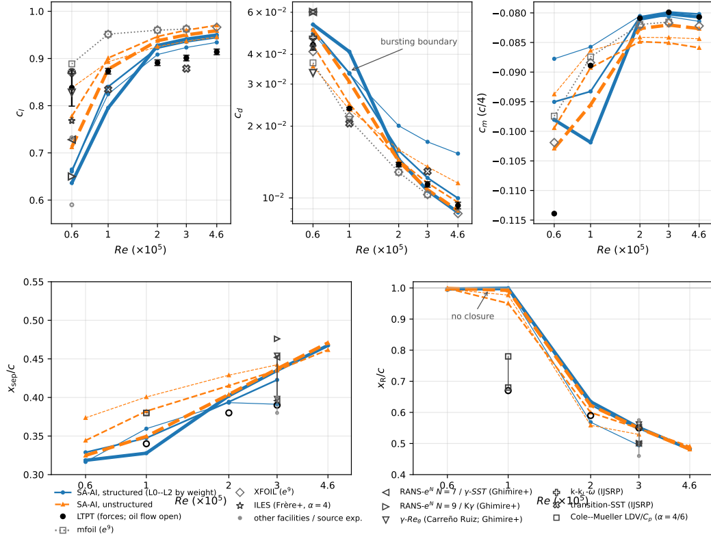
Figure A17: Reynolds-sweep forces and stations.
