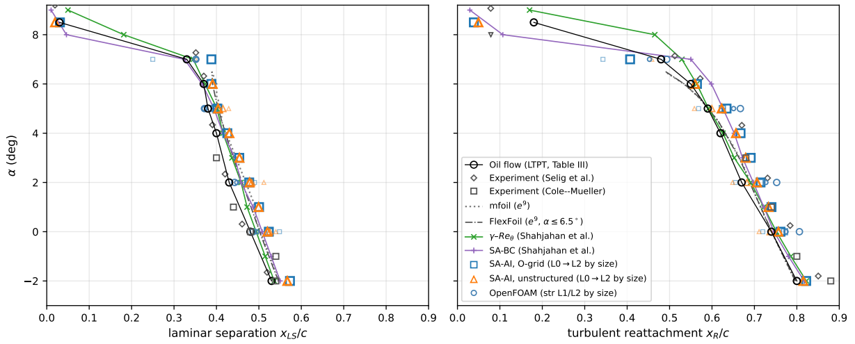
Figure A14: Eppler 387 bubble stations.
