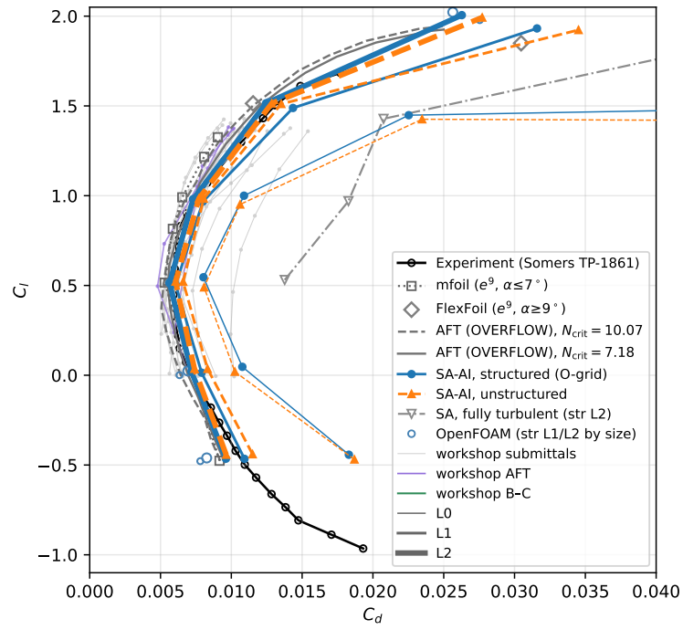
Figure A9: NLF(1)-0416 drag polar.
