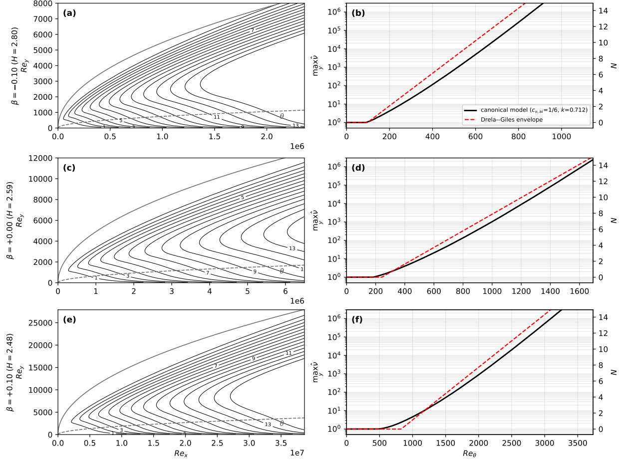
Figure A3: Disturbance transport, three wedges.
