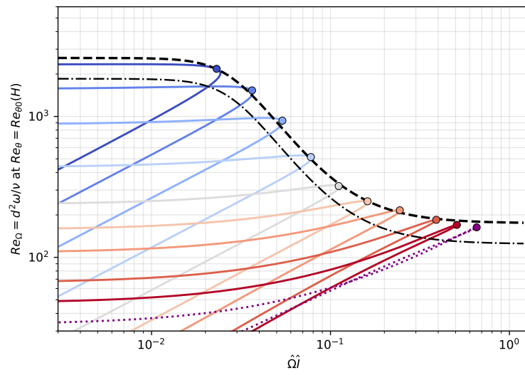
Figure A2: Onset-threshold graze.
