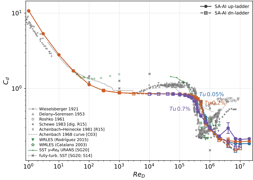
Figure A20: Cylinder drag crisis.
