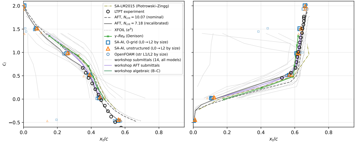
Figure A8: NLF(1)-0416 transition fronts.
