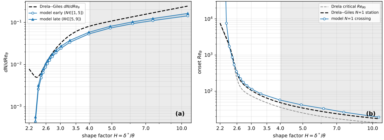
Figure A4: Calibrated model vs Drela-Giles.
