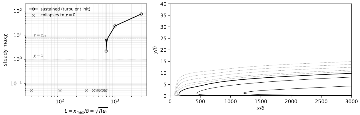
Figure A5: Attachment-anchored turbulent branch.
