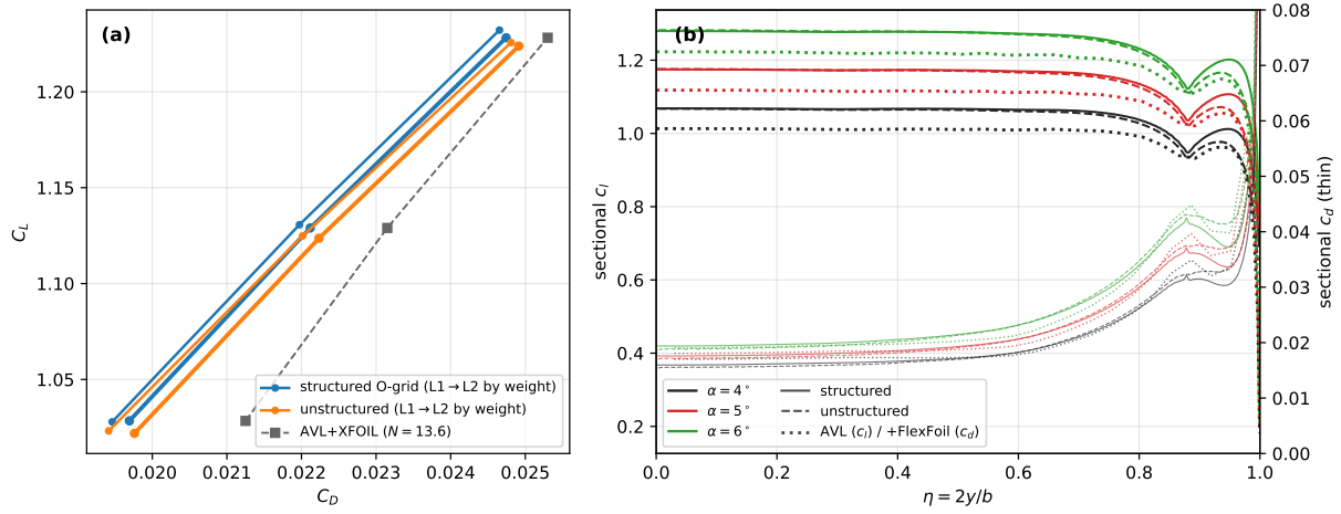
Figure A22: Daedalus polar and sections.
