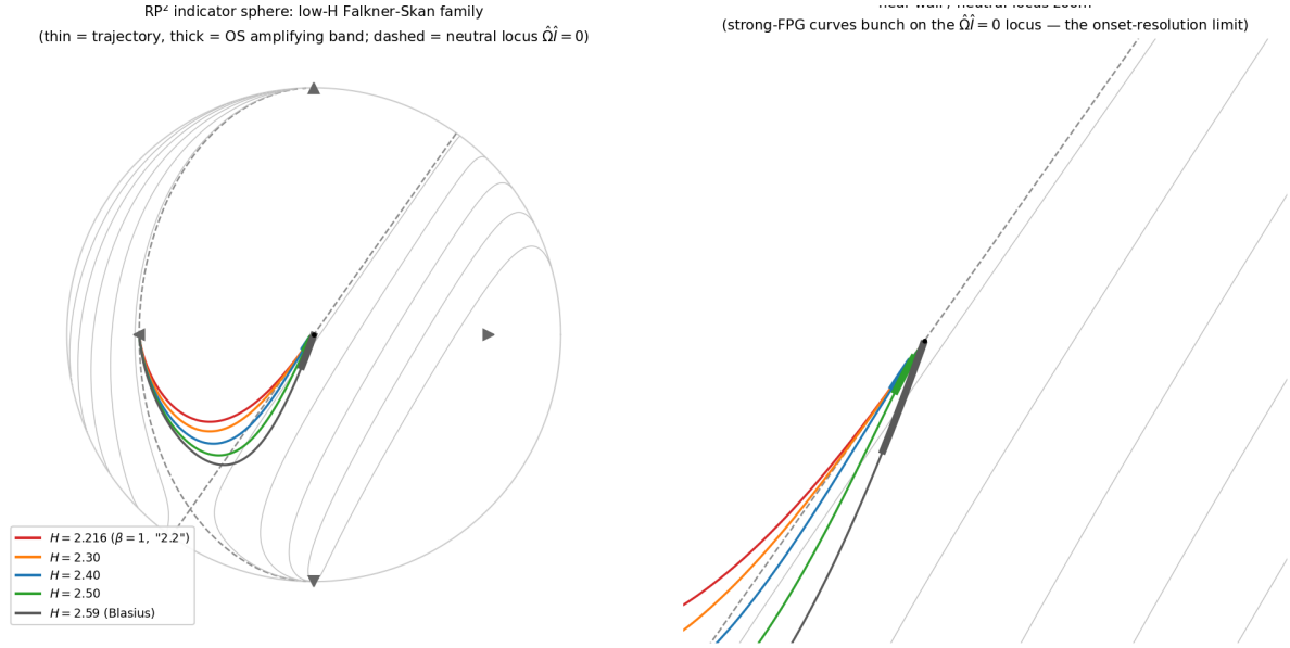
Figure 29: Low- H Falkner-Skan on \mathbb{RP}^2 . H = 2.216 and 2.30 : \max \hat{\Omega}\hat{I} = 1\text{--}3 \times 10^{-4} ( \Delta = 1.6 \times 10^{-4} ), Drela Re_{\theta 0} 6640 vs 3680 ( 1.81\times ).
