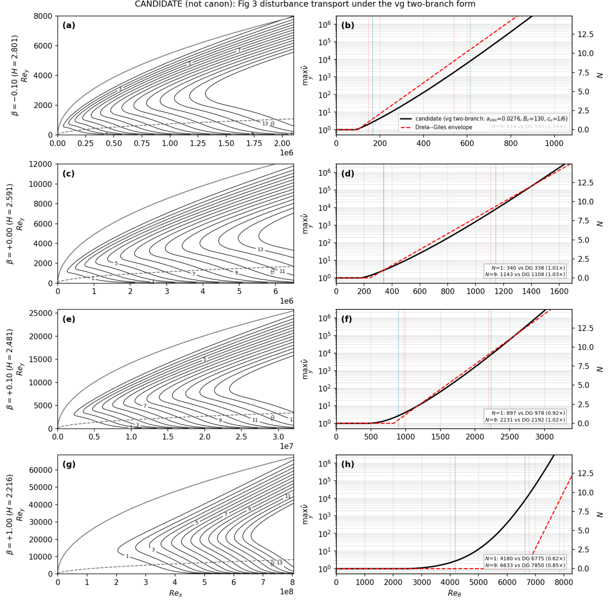
Figure 28: Rows (\beta, H, \max \hat{\Omega} \hat{I}) : (-0.10, 2.80, 0.162) , (0, 2.59, 0.078) , (+0.10, 2.48, 0.037) , (+1.0, 2.22, \sim 2 \times 10^{-4}) . N=1/N=9 vs DG: 1.14/1.14; 1.01/1.03; 0.92/1.02; 0.62/0.85.
