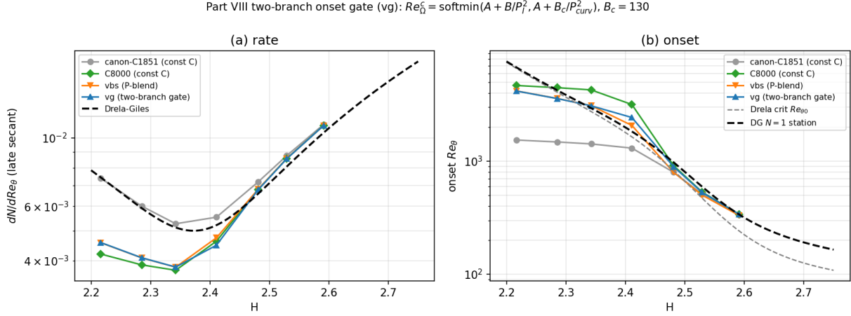
Figure 26: Curves: canon ( C=1851 ), C=8000 , vbs, vg. vg both-panel max 1.63 \times DG; (a) rate; (b) onset on the DG N=1 station to H=2.2 ; low- H rate 0.56 \times DG.
