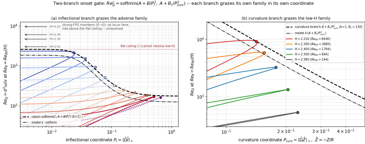
Figure 27: Left P_I (inflectional/adverse family); right P_{\text{curv}} (low- H family). Curvature-branch graze ratio by H : 2.216 \rightarrow 1.00 , 2.30 \rightarrow 0.76 , 2.40 \rightarrow 0.55 , 2.50 \rightarrow 0.29 , 2.59 \rightarrow 0.15 . Drela Re_{\theta_0} : 6640/3680/1794/664/244.
