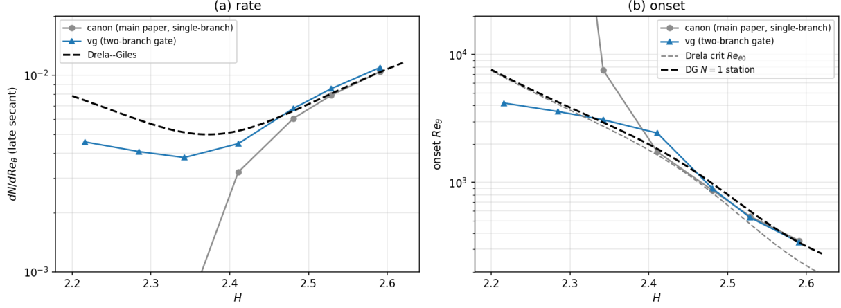
Figure 25: Curves: Drela–Giles, old canon (main-paper single-branch), vg. Canon low- H collapses: onset 369\times DG at H = 2.216 ( 1098\times at 2.285), rate to \sim 0 (both run off-panel); vg tracks DG to 0.6\text{--}1.0\times . (a) rate; (b) onset.
