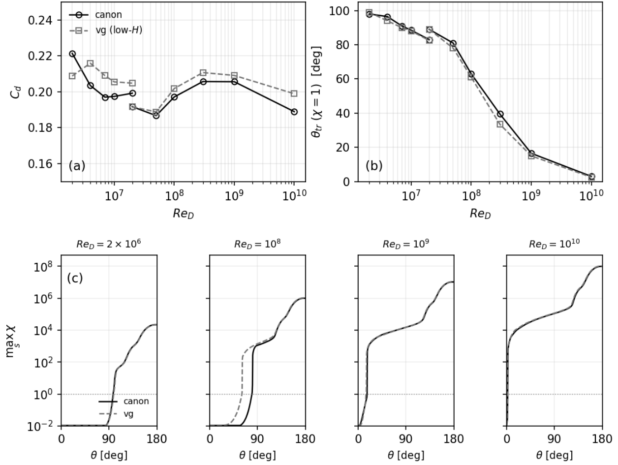
Figure 29: vg (low- H ) vs canon, Tu = 0.2\% up-ladder, Re_D = 2 \times 10^6 - 10^{10} (highre mesh \leq 2 \times 10^7 , ultra \geq 2 \times 10^7 ). (a) C_d : both 0.19–0.22, vg +3–6%; neither reaches the transcritical 0.5–0.7. (b) \theta_{tr} (\chi = 1) : front advances 98^\circ \rightarrow 2.5^\circ ; vg tracks canon within 6^\circ .
