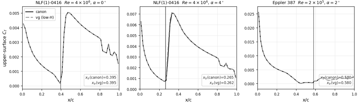
Figure 30: Upper-surface C_f(x/c) , canon (black) vs vg low- H (gray dashed), kernel-only delta (same mesh/config/seed, vg warm-restarted from canon). Vertical ticks: transition front (near-wall \chi = 1 for NLF, C_f -rise for Eppler). Curves and fronts overlap: NLF(1)-0416 Re = 4 \times 10^6 \alpha = 0^\circ x_{tr} = 0.395 (both), \alpha = 4^\circ 0.265 \rightarrow 0.262 ; Eppler 387 Re = 2 \times 10^5 \alpha = 2^\circ 0.580 (both). The low- H branch does not trip the favorable rooftop.
