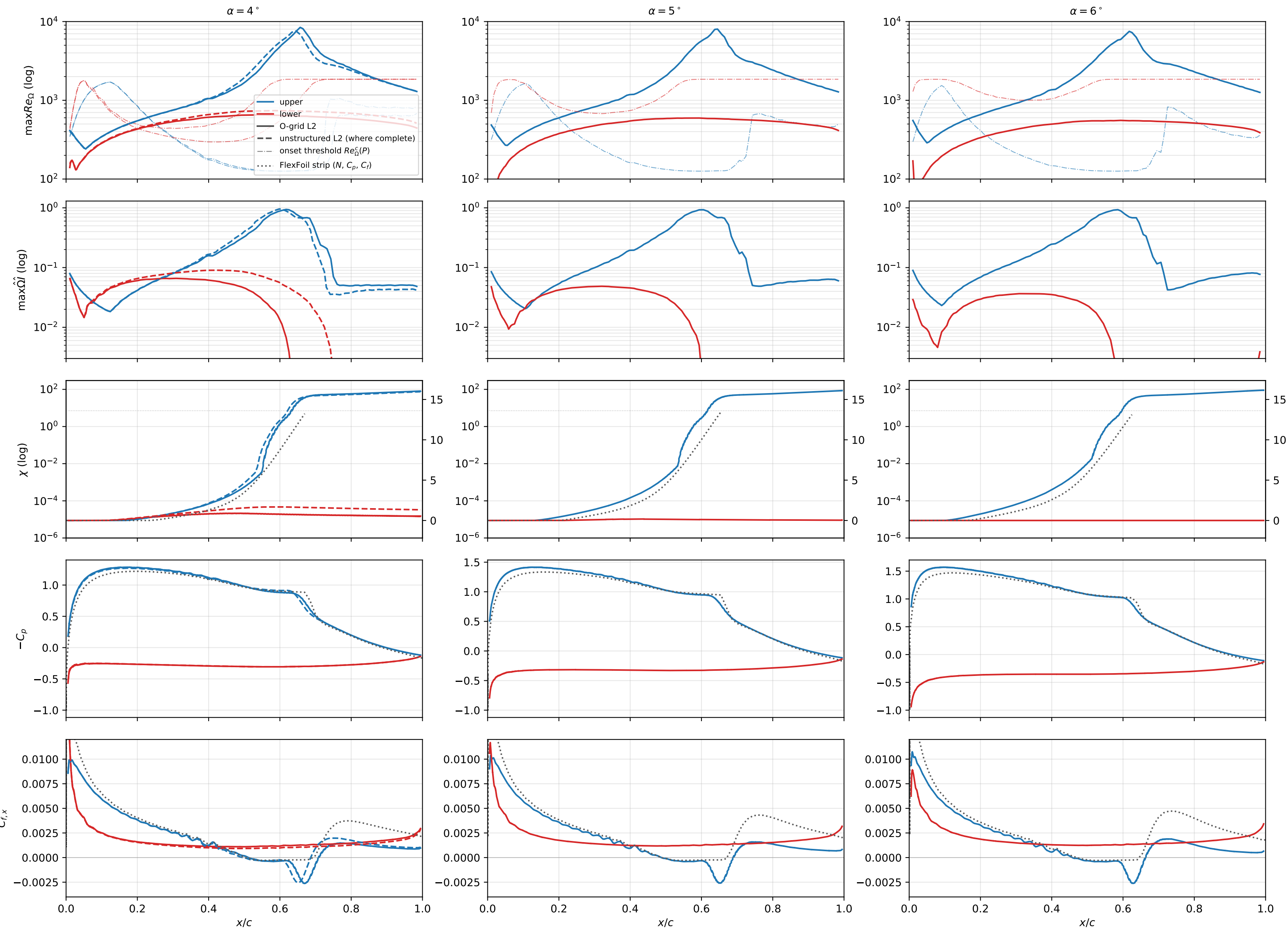
Daedalus wing section \eta = 0.75 ( Re_c = 5e + 05 )
