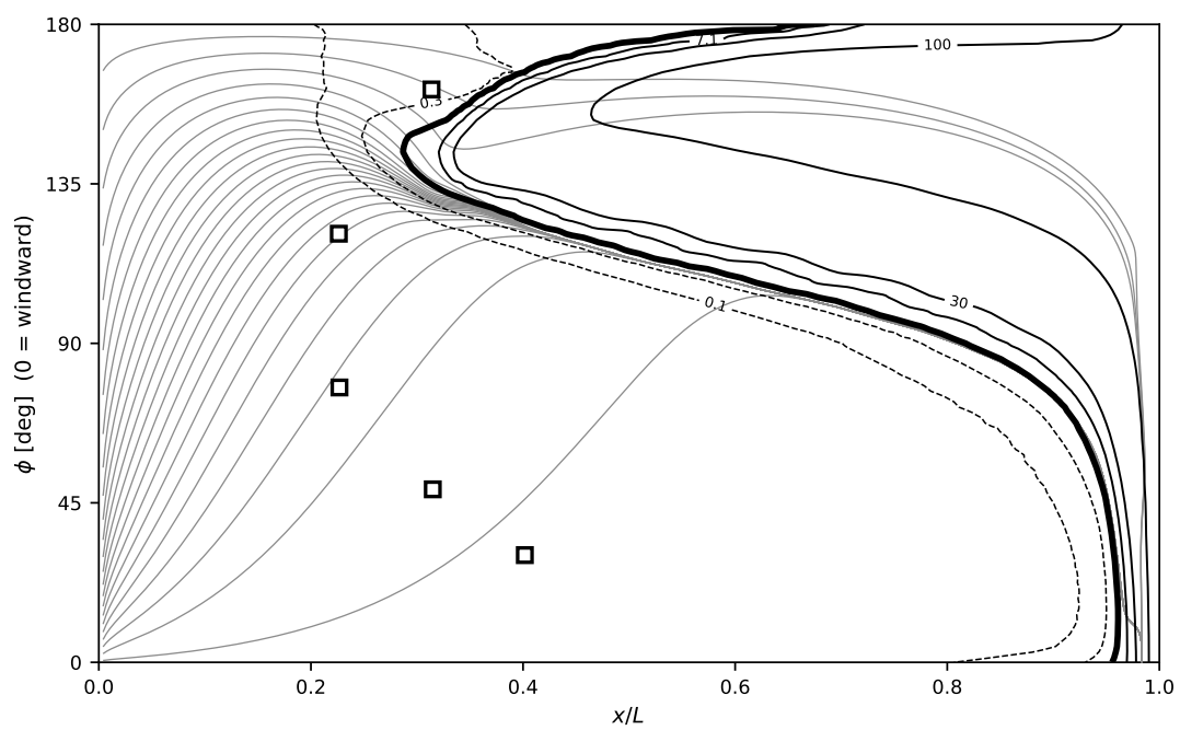
Fig. 34 \alpha = 10^\circ , Re_L = 6.56 \times 10^6 , ONERA F1 seed; the condition differs from its Göttingen twin only in the freestream seed.
