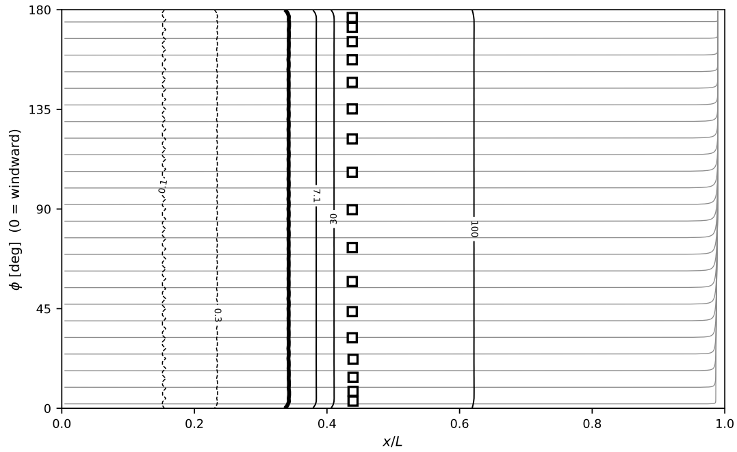
Fig. 30 Surface unrolled into (x/L, \phi) , \phi=0 the windward symmetry line, at the measured-seed condition. Grey: skin-friction lines integrated from the wall shear vector itself—the oil-flow analogue, and not the inviscid streamlines of Stock Figs. 14–17—whose convergence marks separation. Black: the \max_n \chi family on a wall-normal segment shot from each surface point, sub-unity decades dashed, \chi=1 heavy, \chi=c_{v1} and above solid. White-filled squares: the measured DFVLR transition points. Zero incidence, Re_L=7.2\times 10^6 : both families are functions of x/L alone, as the axisymmetric flow requires.
