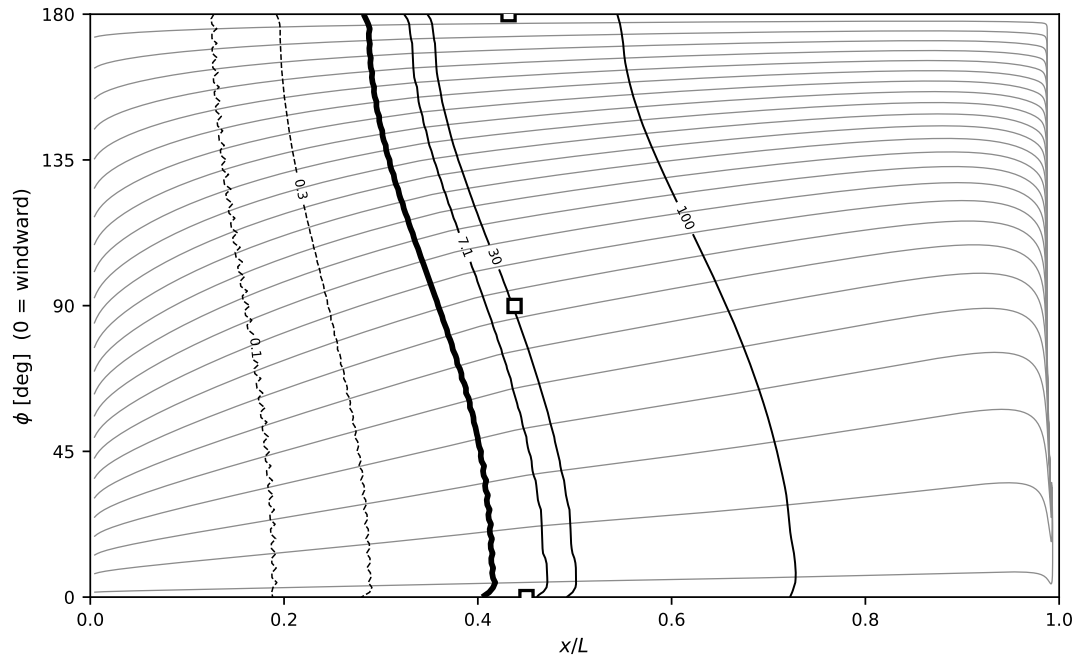
Fig. 31 \alpha=2.5^\circ , Re_L=7.2\times 10^6 .
