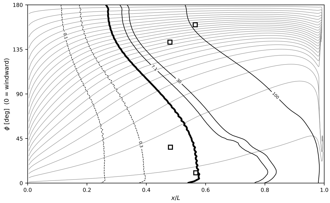
Fig. 32 \alpha = 5^\circ , Re_L = 6.49 \times 10^6 .
