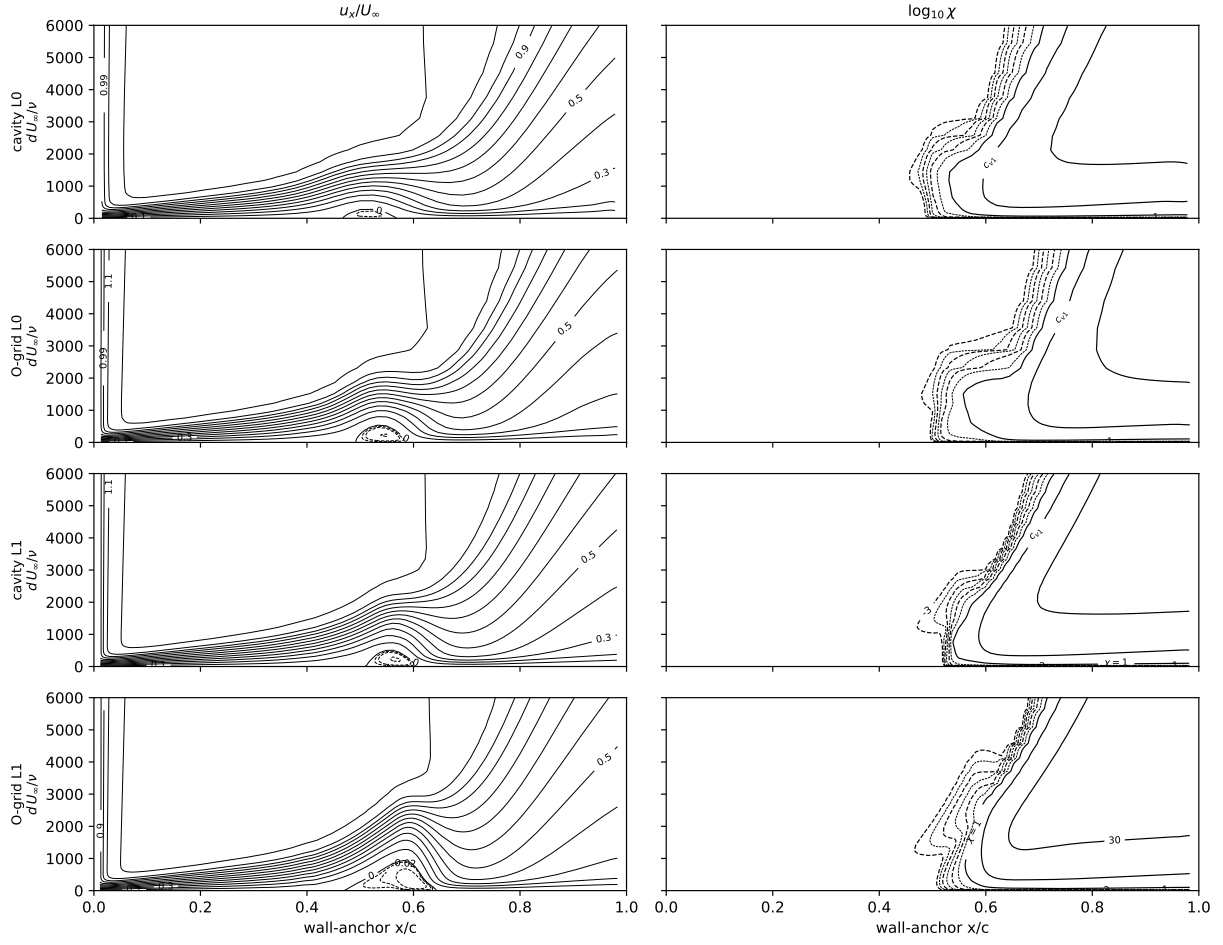
Fig. D10 As Fig. D9, at \eta = 0.75 .
