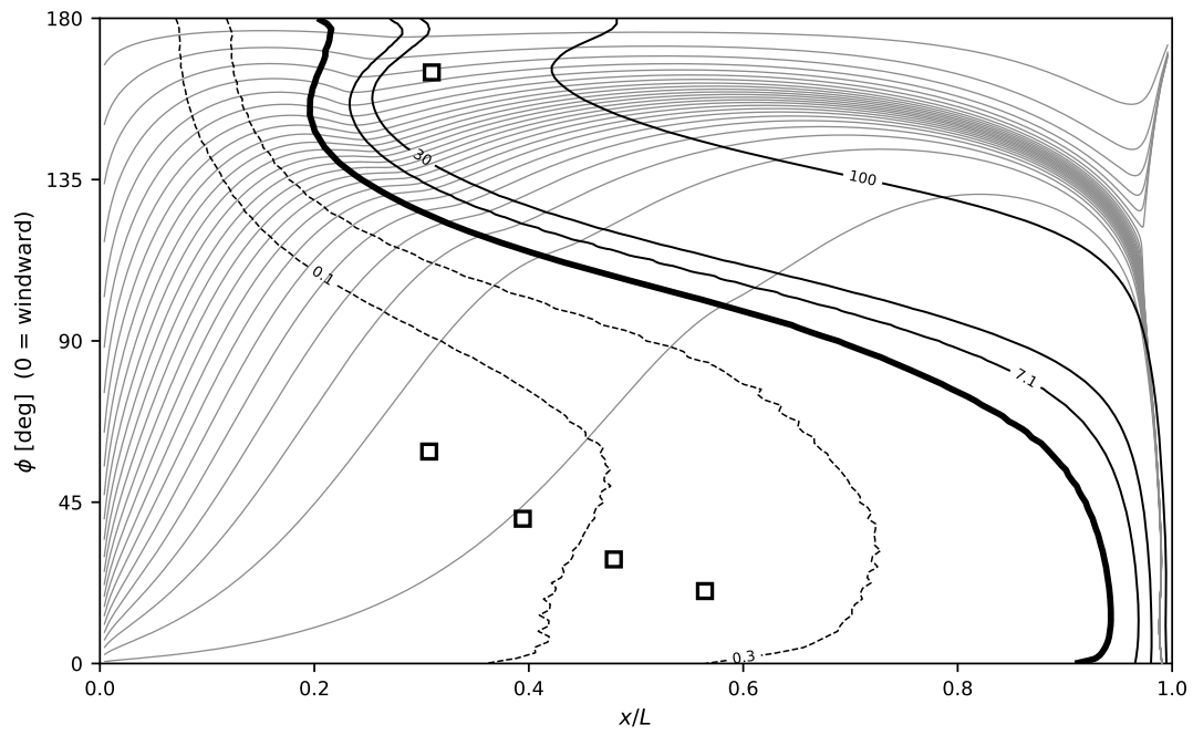
Fig. 33 \alpha = 10^\circ , Re_L = 6.56 \times 10^6 , Göttingen seed.
