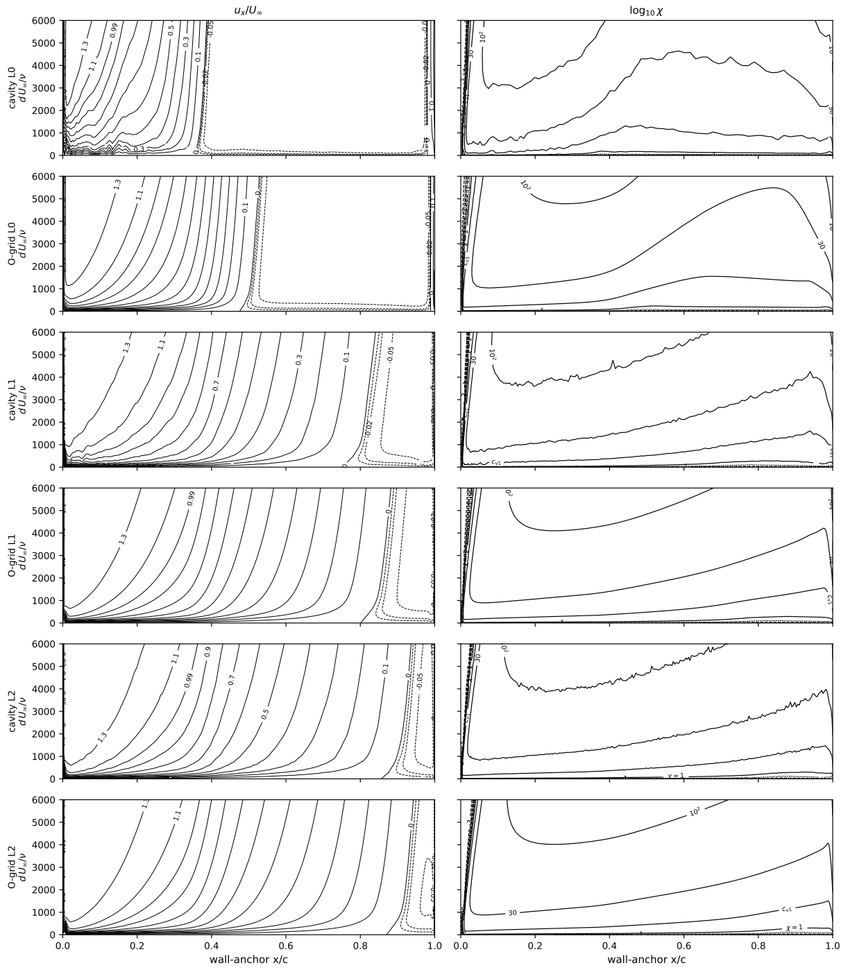
Fig. A13 NLF(1)-0416, Re = 4 \times 10^6 , \alpha = 15^\circ , upper surface: streamwise velocity u_x/U_\infty (left) and \log_{10} \chi (right) on all six grids.
