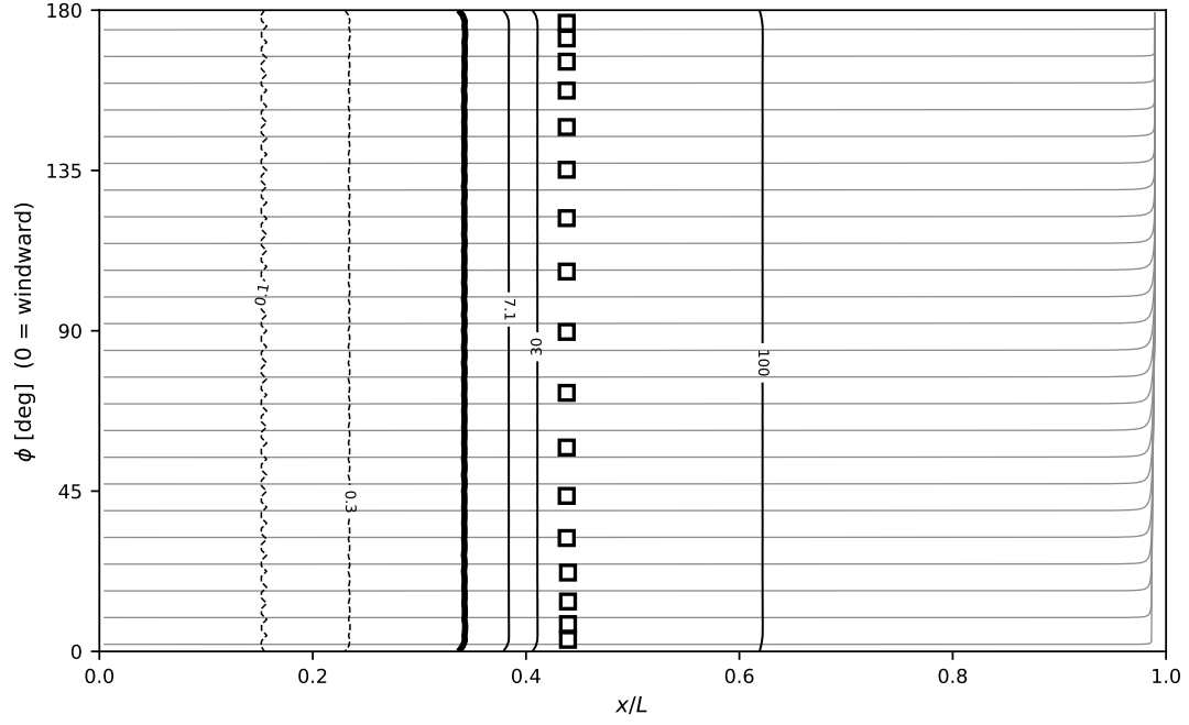
Figure 28: \alpha = 0^\circ , Re_L = 7.2 \times 10^6 .
