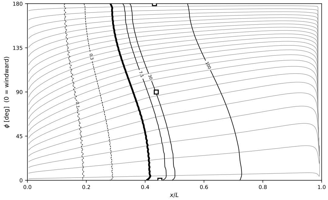
Figure 29: \alpha = 2.5^\circ , Re_L = 7.2 \times 10^6 .
