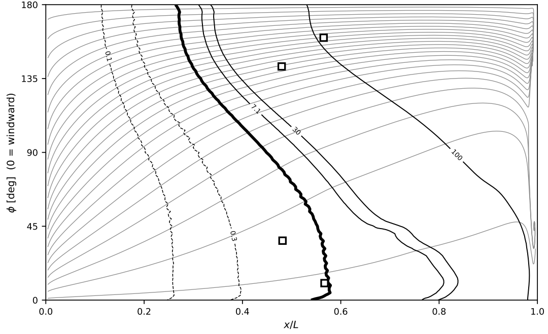
Figure 30: \alpha = 5^\circ , Re_L = 6.49 \times 10^6 .
