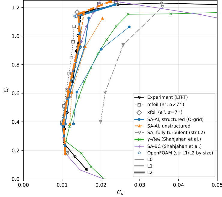
Fig. 11 Drag polar of the Eppler 387 at Re=2\times 10^5 : the present SA-AI prediction (all six grids at \alpha \in \{0^\circ, 2^\circ, 5^\circ, 7^\circ\} ; the finest L2 pair extended over \alpha = -2^\circ – 8.5^\circ with the six additional computed incidences) overlaid on the digitized experimental section characteristics from the Langley Low-Turbulence Pressure Tunnel (McGhee et al., NASA TM-4062, App. B, R=2\times 10^5 ) and the mfoil e^9 reference, spanning the same extended incidence range (XFOIL fills \alpha=7^\circ , where mfoil’s coupled solve fails). The computed points track the low-drag laminar bucket; the two mesh families agree to within \Delta C_d \leq 2.4 \times 10^{-4} across \alpha = -2^\circ – 7^\circ and to 1.0 \times 10^{-3} at the unsteady 8.5^\circ point. The gray dash-dot curve is fully turbulent SA ( \chi_\infty=3 , same solver, structured L2 grid), 77–97% above the SA-AI drag in the bucket and +151% at \alpha=7^\circ . The green and purple curves are the \gamma – Re_\theta (Langtry–Menter, OpenFOAM) and SA-BC (SU2) transition models at the same condition and Tu=0.1\% , digitized from Ref. [39] (Appendix F); the SA-BC intermittency correlation was calibrated in part on this airfoil [40]. Small steel-blue circles: the independent cell-centered incompressible (OpenFOAM) implementation on the structured L1/L2 grids (by size), as in Fig. 7; the port omits the bypass of Eq. 18, worth -6 to -10 counts at \alpha=0 – 5^\circ here, and drag agreement is not claimed—the visible offsets are consistent with that omission in sign and magnitude (Table F6).
