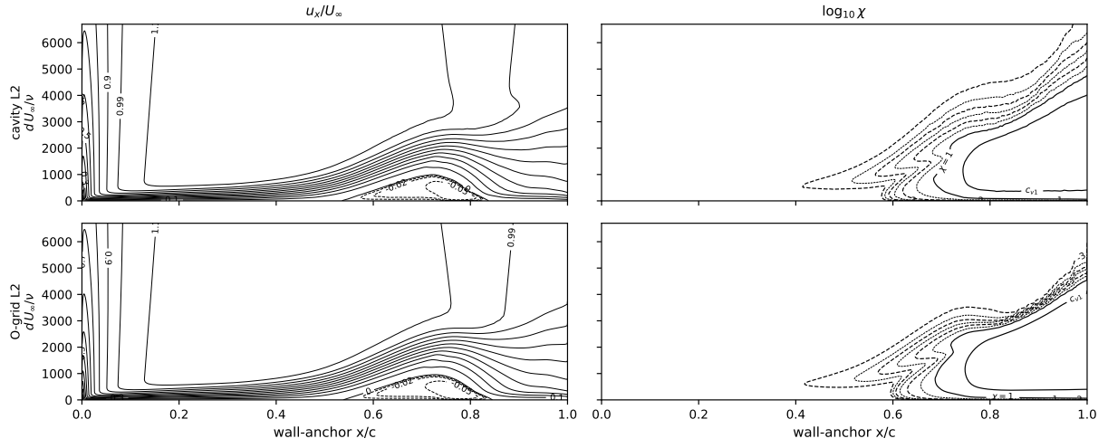
Fig. B1 Eppler 387, Re = 2 \times 10^5 , \alpha = -2^\circ , upper surface (finest L2 pair; the extension incidences exist on L2 only): streamwise velocity u_x/U_\infty (left) and \log_{10} \chi (right). The bubble sits at its aft-most station of the sweep ( x/c \approx 0.55\text{--}0.80 ).
