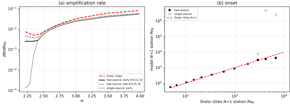
Fig. H5 Two-source rate against Drela–Giles across the Falkner–Skan family, \beta = +1.0 (stagnation, H \approx 2.22 ) to -0.1988 (incipient separation, H = 3.98 ); analytic march, no CFD. (a) amplification rate as early ( N \in [1, 5] ) and late ( N \in [5, 9] ) secants, with the single-source rate for comparison—the low- H collapse is the deficit the viscous branch removes. (b) the marched N = 1 station against the Drela–Giles N = 1 station Re_{\theta 0} + 1/(dN/dRe_\theta) ; the diagonal is exact agreement.
