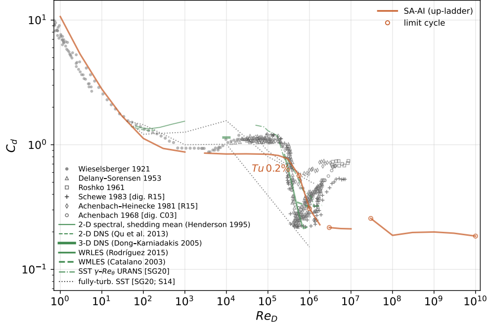
Fig. 18 Steady-branch drag coefficient of the circular cylinder, Re_D = 1-10^{10} : the single freestream seed ( Tu=0.2\% , \chi_\infty from Mack’s map), swept as an upward continuation ladder in Re_D over four contiguous grid families, overlaid on the experimental and computational literature. Open rings mark the cases the steady monitor did not accept (peak-to-peak in Table F8). Below Re_D \approx 46 the steady solution is the physical flow; between there and \sim 10^3 the steady-branch points are drawn for continuity, not validation. Symbols are experiments; lines are computations. Gray and black symbols, digitized independently from the sources: Wieselsberger’s nine-diameter composite [57] (faired low- Re_D curve rendered as sparse symbols along its polyline), Delany & Sorensen [58], Roshko’s pressurized-tunnel points (splitter-plate runs excluded) [59], Schewe [54] and Achenbach & Heinecke [62] as replotted by Rodríguez et al. [51], the Achenbach drag curve [49] as reproduced by Catalano et al. [60] (likewise sparse symbols), and the low- Re_D laminar drag collected by Veysey & Goldenfeld [63]. Green lines are transition-resolving computations. In the shedding band the unsteady two-dimensional shedding-mean drag—Henderson’s spectral-element curve [64] (solid) and the DNS sweep of Qu et al. [65] (dashed)—recovers the measured level exactly where the steady branch reported here sits below it by construction. At the crisis: wall-resolved LES [51] (solid), wall-modeled LES [60] (dashed), and the SST \gamma-Re_\theta transition URANS sweep of Stabnikov & Garbaruk [61] (dash-dotted); the short green stub at Re_D = 10^4 marks the finest-grid value of the three-dimensional spectral DNS of Dong & Karniadakis [66] (its N_z \geq 64 resolution study brackets C_d = 1.110-1.143 ). Charcoal dotted lines are fully-turbulent SST URANS [61, 67]. The steady solutions lie below the shedding-mean experimental band at subcritical Re_D by construction; the comparison targets the crisis location and the supercritical level. Every SA-AI point is tabulated in Table F8; digitization provenance in repro/cfd/litdata/dragcrisis/.
