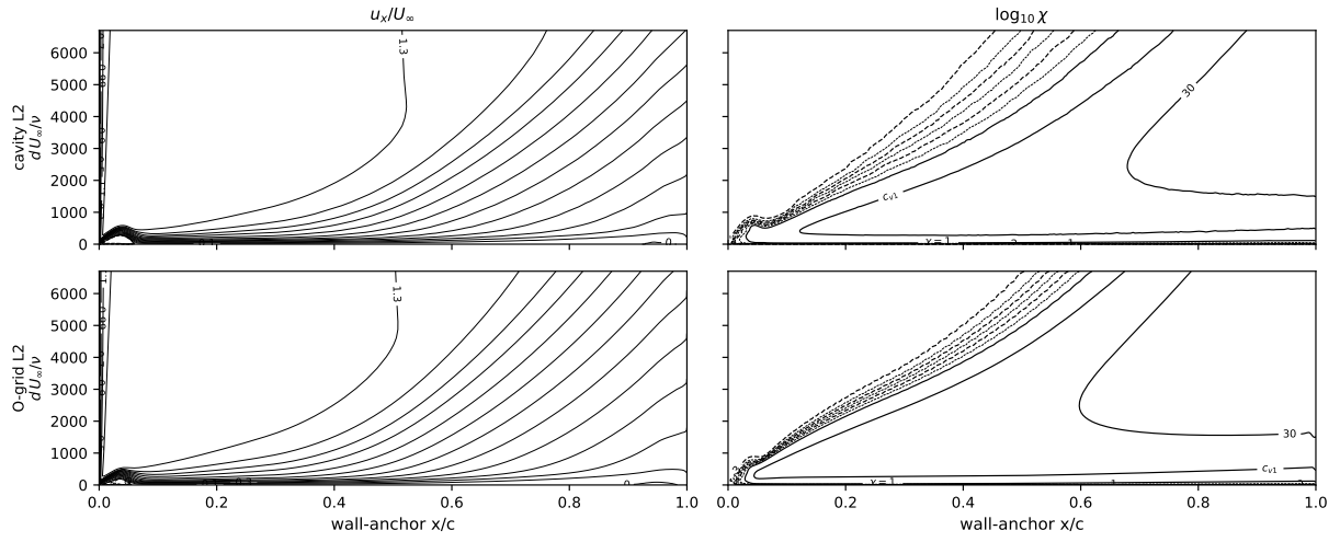
Fig. B6 Eppler 387, Re = 2 \times 10^5 , \alpha = 8.5^\circ , upper surface (finest L2 pair): streamwise velocity u_x/U_\infty (left) and \log_{10} \chi (right). Past the experimental stall: the layer trips in the leading-edge bubble within the first few percent of chord—closing roughly 4\times shorter than the measured 0.03\text{--}0.18\,c recovery (Fig. 14)—and runs turbulent and attached over the rest of the surface (Fig. 13).
