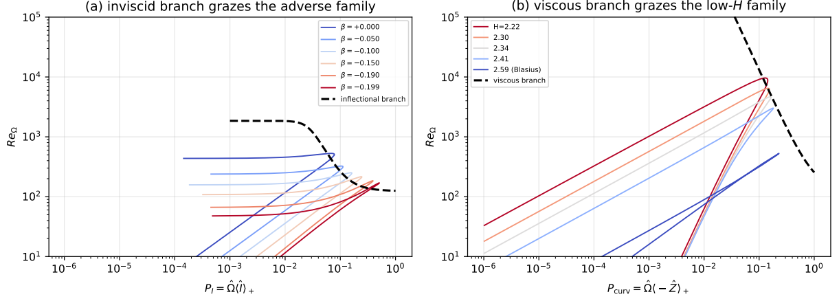
Figure 34: Each onset branch grazes its own family in its own coordinate, each profile evaluated at its Drela–Giles critical Reynolds number Re_{\theta 0}(H) . (a) the inflectional branch A + B/P_I^2 against the adverse family; the strongly favorable members collapse to P_I \rightarrow 0 and leave the panel, which is the onset-resolution limit of a single-coordinate gate. (b) the curvature branch A + B_c/P_c^2 against exactly those low- H members, in the coordinate P_c of Eq. (14).
