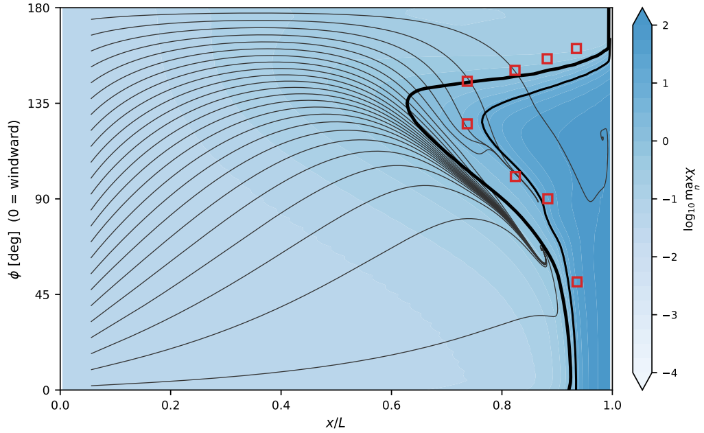
Figure 38: \alpha = 5^\circ , Re_L = 1.52 \times 10^6 .
