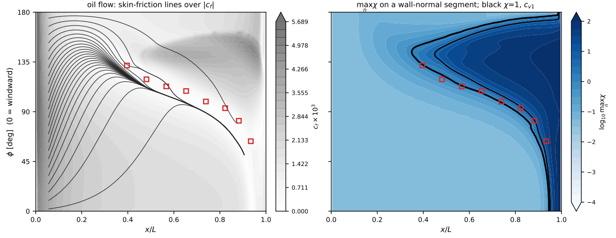
Figure 30: \alpha = 10^\circ , Re_L = 1.52 \times 10^6 .
