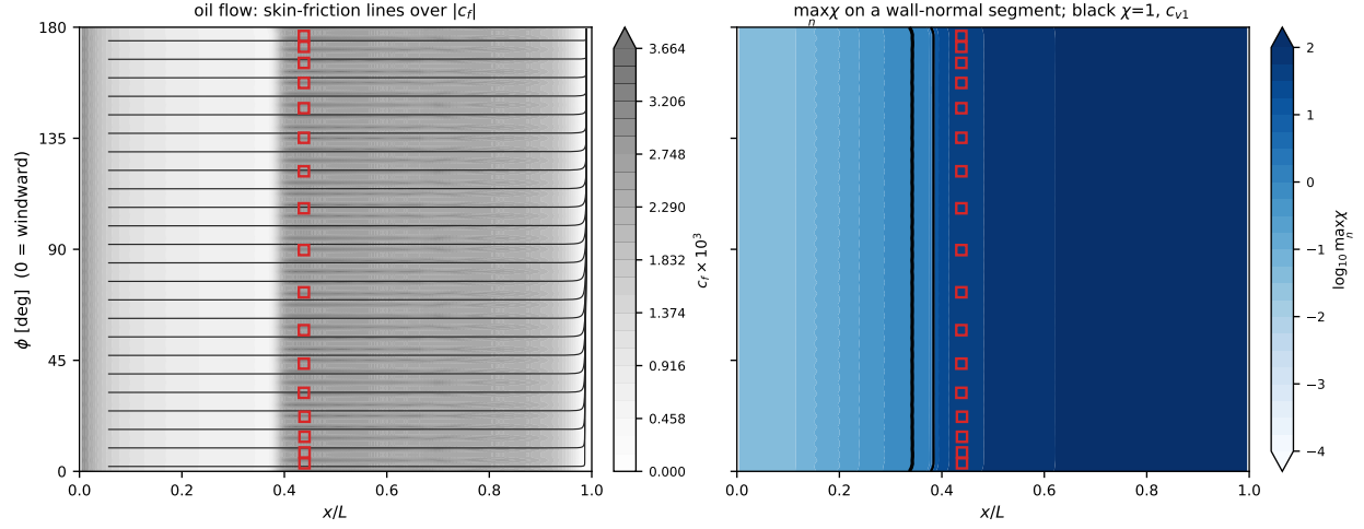
Figure 26: Surface at the measured-seed condition, unrolled into (x/L, \phi) , \phi = 0 windward. Left: skin-friction lines integrated from the wall shear vector over filled |c_f| – the oil-flow analogue, and not the inviscid streamlines of Stock Figs. 14–17. Right: \max_n \chi on a wall-normal segment from each surface point, black contours \chi = 1 and \chi = c_{v1} . Open red squares: measured DFVLR transition. \alpha = 0^\circ , Re_L = 7.2 \times 10^6 .
