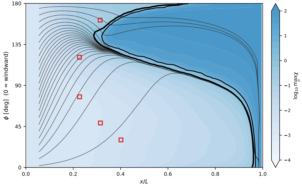
Figure 42: \alpha = 10^\circ , Re_L = 6.56 \times 10^6 , ONERA F1.
