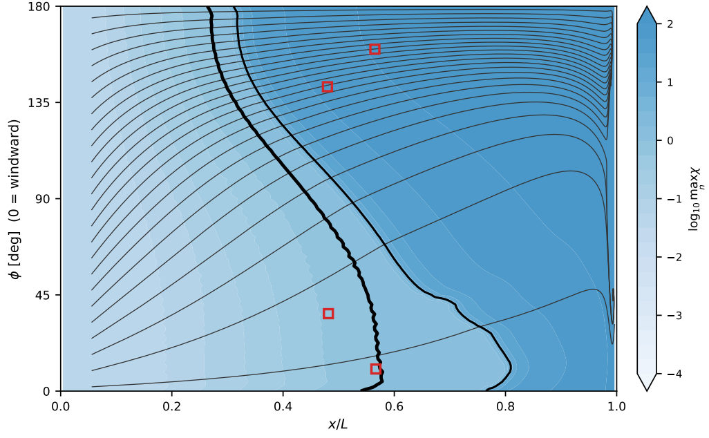
Figure 39: \alpha = 5^\circ , Re_L = 6.49 \times 10^6 .
