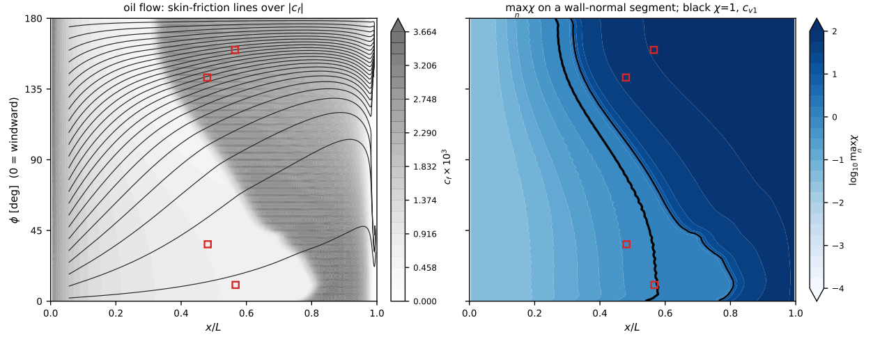
Figure 29: \alpha = 5^\circ , Re_L = 6.49 \times 10^6 .
