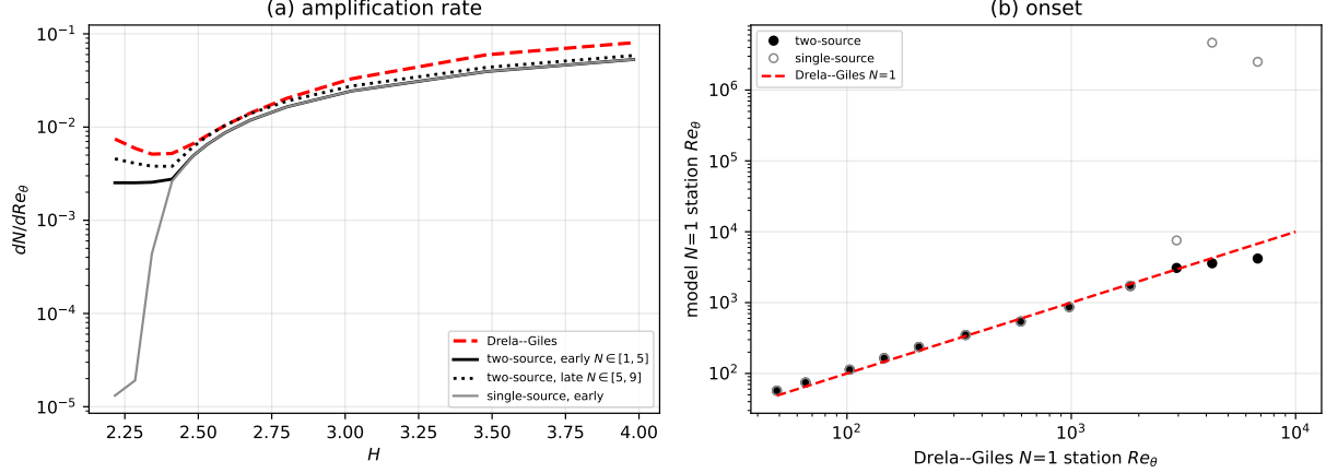
Figure 33: Two-source rate against Drela–Giles across the Falkner–Skan family, \beta = +1.0 (stagnation, H \approx 2.22 ) to -0.1988 (incipient separation, H = 3.98 ); analytic march, no CFD. (a) amplification rate as early ( N \in [1, 5] ) and late ( N \in [5, 9] ) secants, with the single-source rate for comparison—the low- H collapse is the deficit the viscous branch removes. (b) the marched N = 1 station against the Drela–Giles N = 1 station Re_{\theta 0} + 1/(dN/dRe_{\theta}) ; the diagonal is exact agreement.
