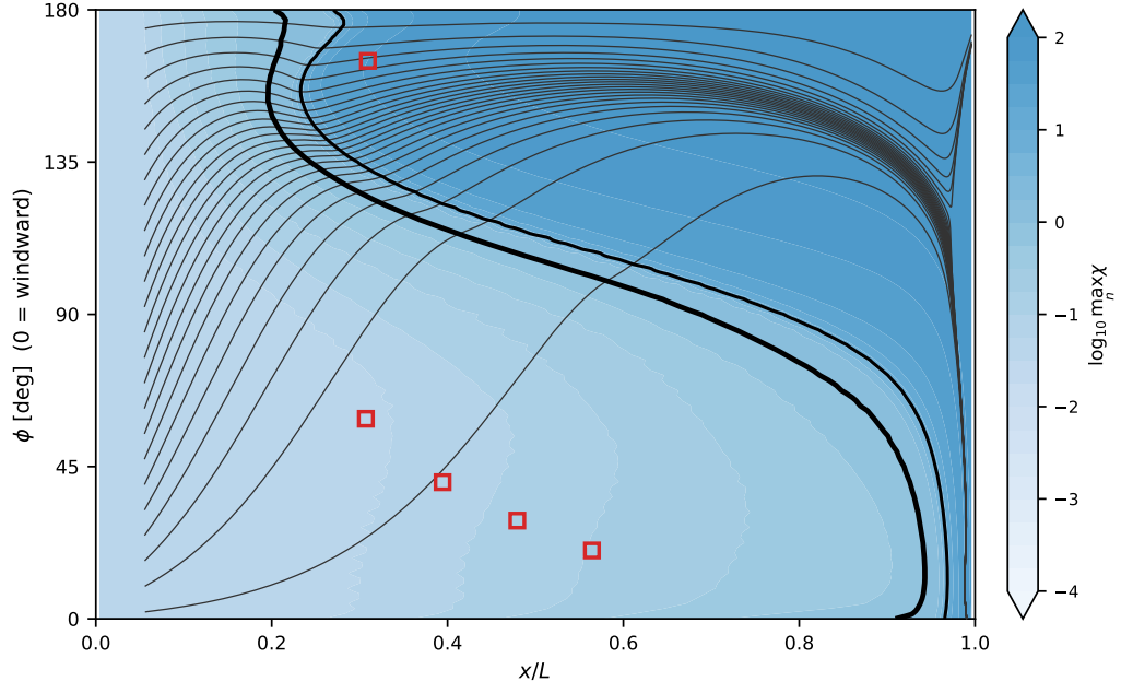
Figure 41: \alpha = 10^\circ , Re_L = 6.56 \times 10^6 , Göttingen.
