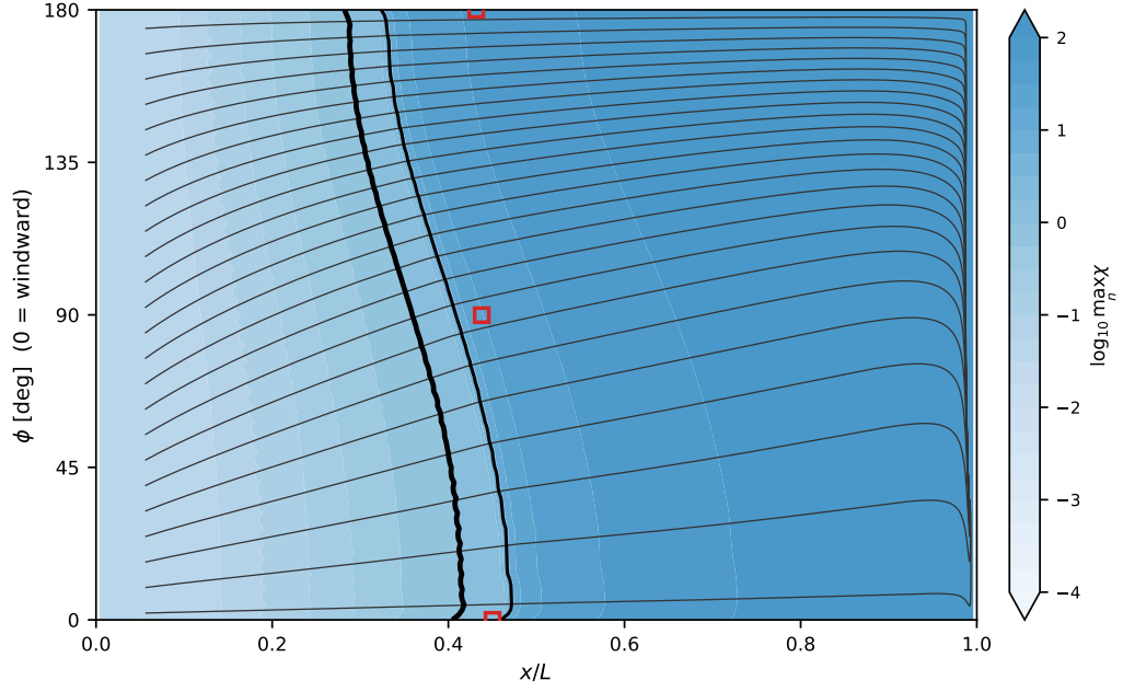
Figure 37: The two views superposed, inclined conditions. Filled \log_{10} \max_n \chi (ramp truncated light so the streaks read over it), skin-friction lines dark grey, \chi = 1 and \chi = c_{v1} heavy black, measured DFVLR transition open red. Zero incidence is omitted: both views are functions of x/L alone there. \alpha = 2.5^\circ , Re_L = 7.2 \times 10^6 .
