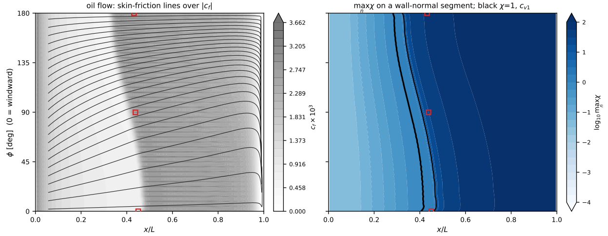
Figure 27: \alpha = 2.5^\circ , Re_L = 7.2 \times 10^6 .
