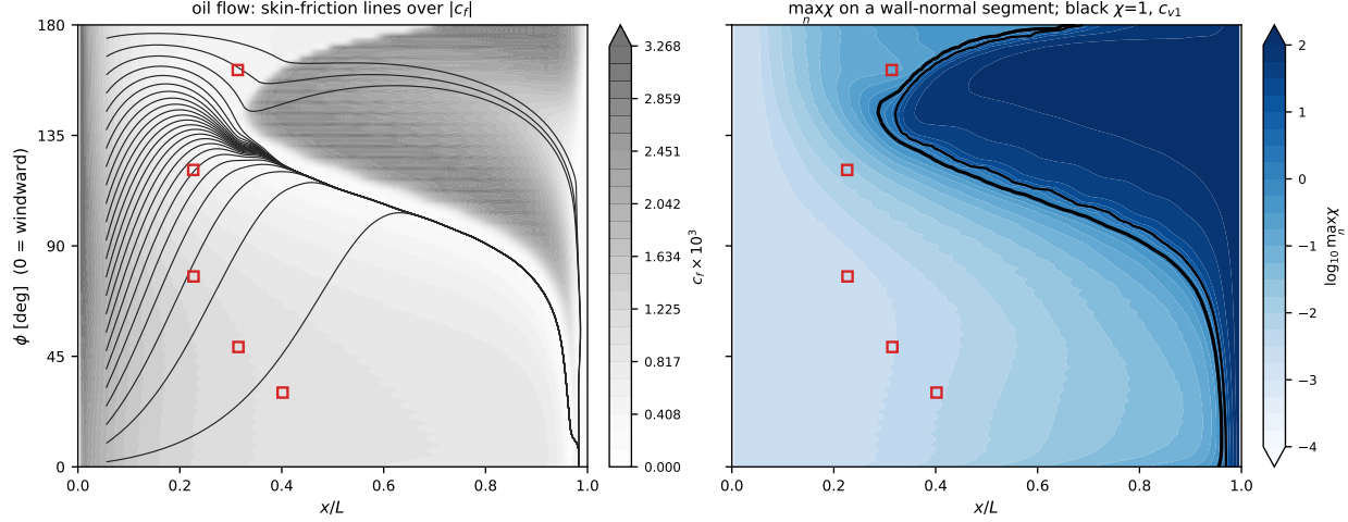
Figure 32: \alpha = 10^\circ , Re_L = 6.56 \times 10^6 , ONERA F1.
