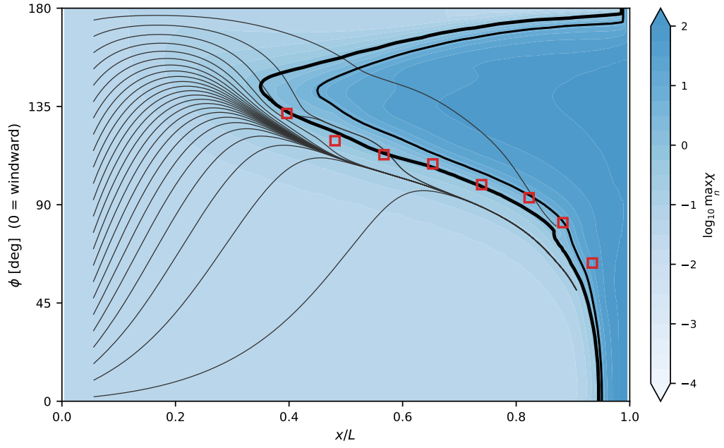
Figure 40: \alpha = 10^\circ , Re_L = 1.52 \times 10^6 .
