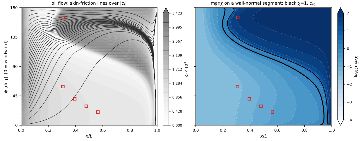
Figure 31: \alpha = 10^\circ , Re_L = 6.56 \times 10^6 , Göttingen.
