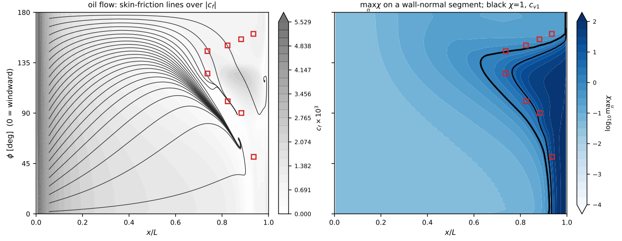
Figure 28: \alpha = 5^\circ , Re_L = 1.52 \times 10^6 .
