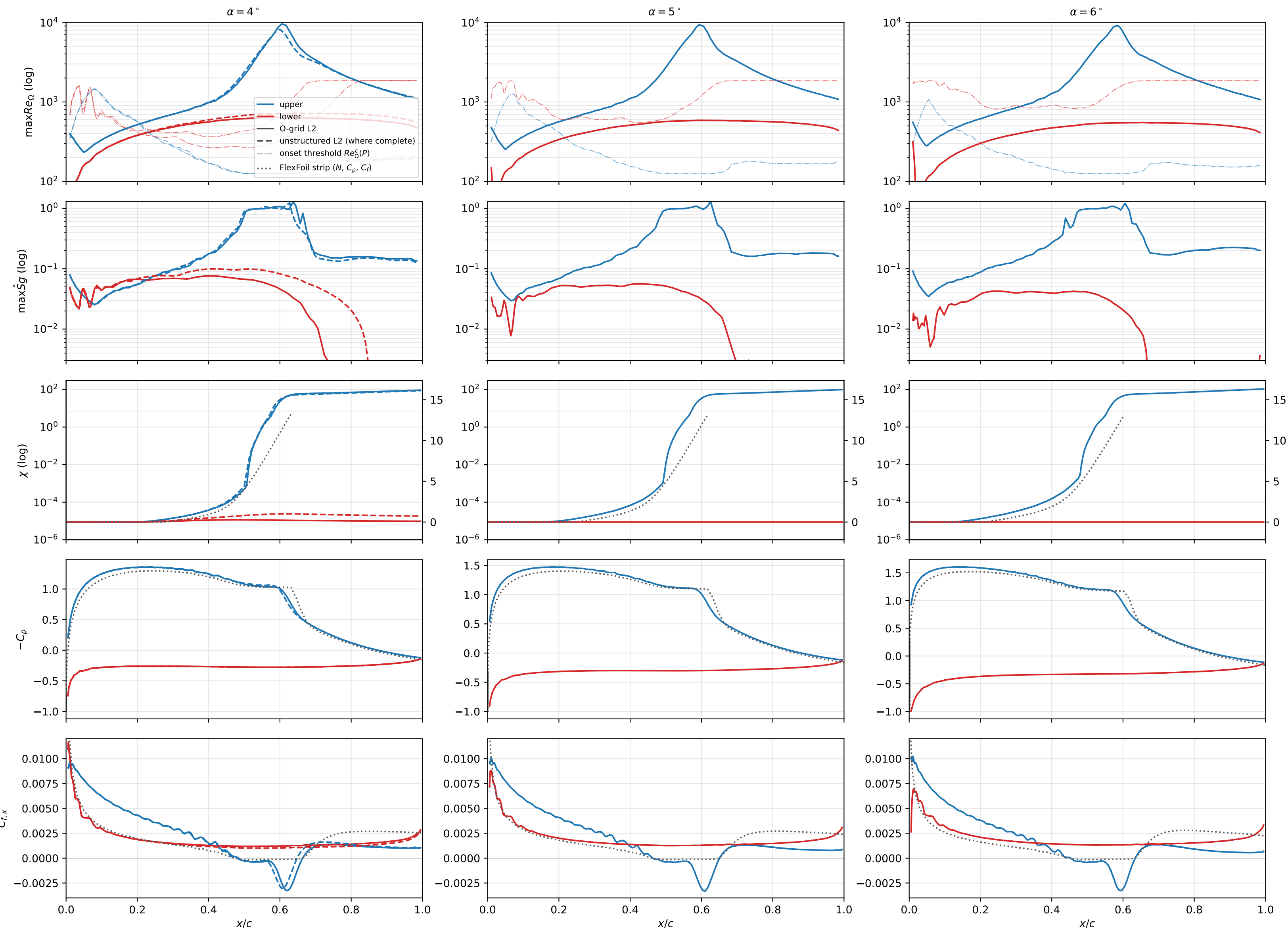
Daedalus wing section \eta = 0.31 ( Re_c = 5e + 05 )
