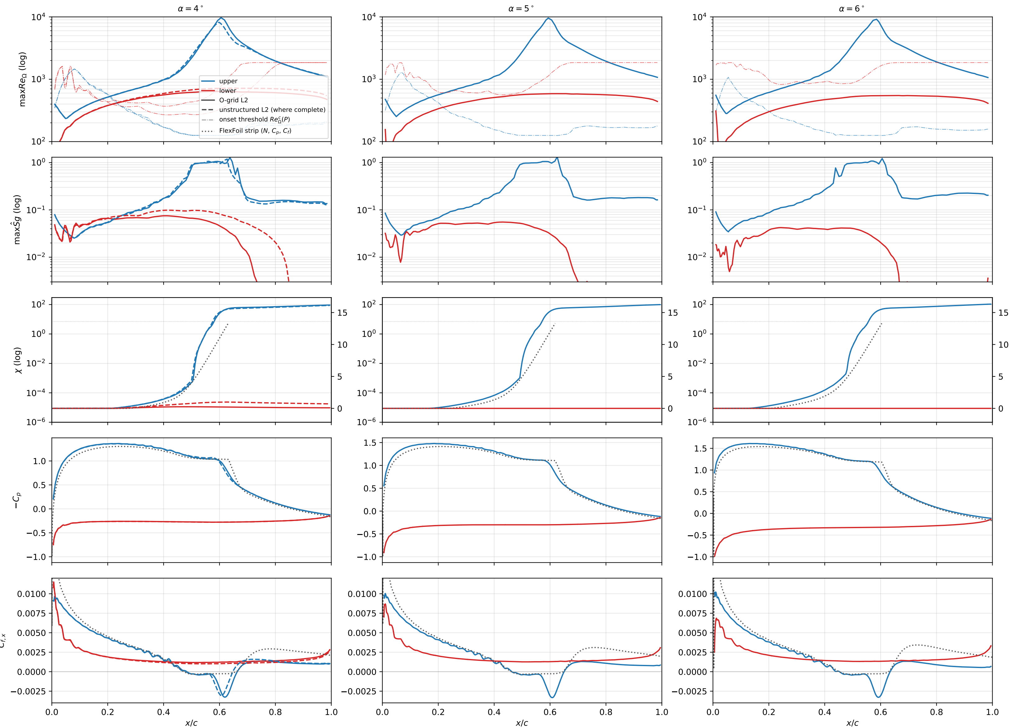
Daedalus wing section \eta = 0.10 ( Re_c = 5e + 05 )
