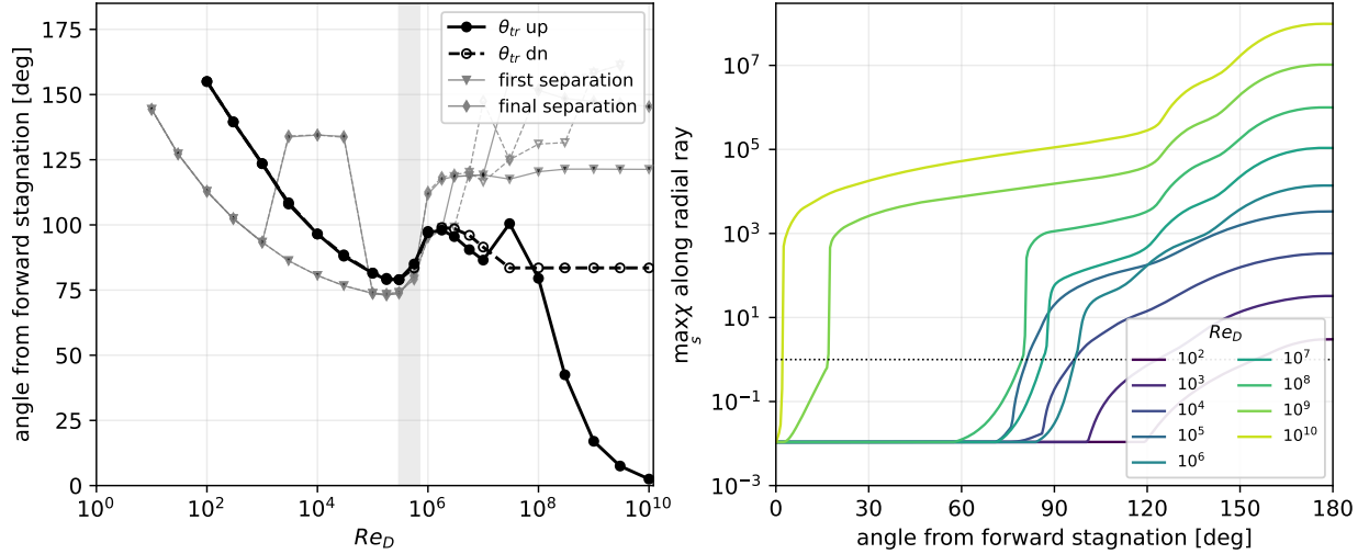
Figure 21: Tu = 0.2\% , Re_D = 1-10^{10} . (a) transition angle \theta_{tr} ( \chi = 1 ; up solid, down dashed) and first/final wall separation vs Re_D (below the crisis \theta_{tr} is the wake \chi = 1 front); the front marches from \sim 100^\circ to \sim 2^\circ by 10^{10} . (b) \max_s \chi(\theta) per decade 10^2-10^{10} (up-ladder).
