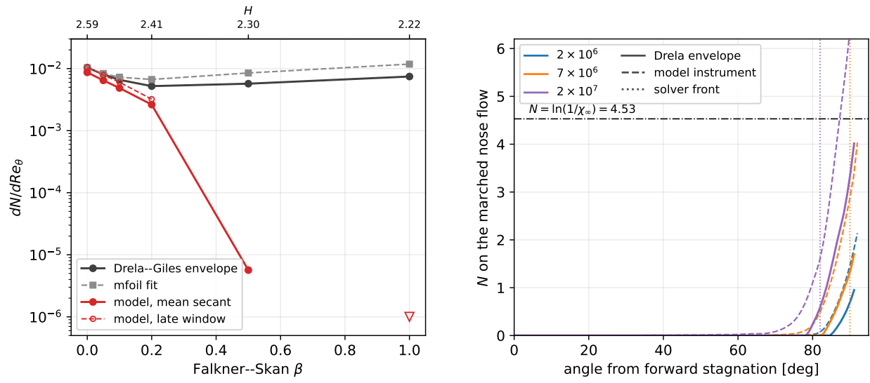
Figure 22: Favorable-gradient amplification audit.
