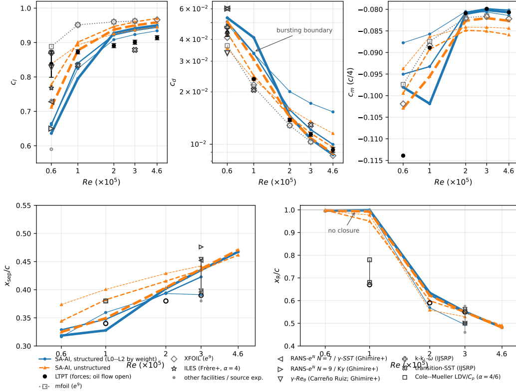
Figure 17: Reynolds-sweep forces and stations.
