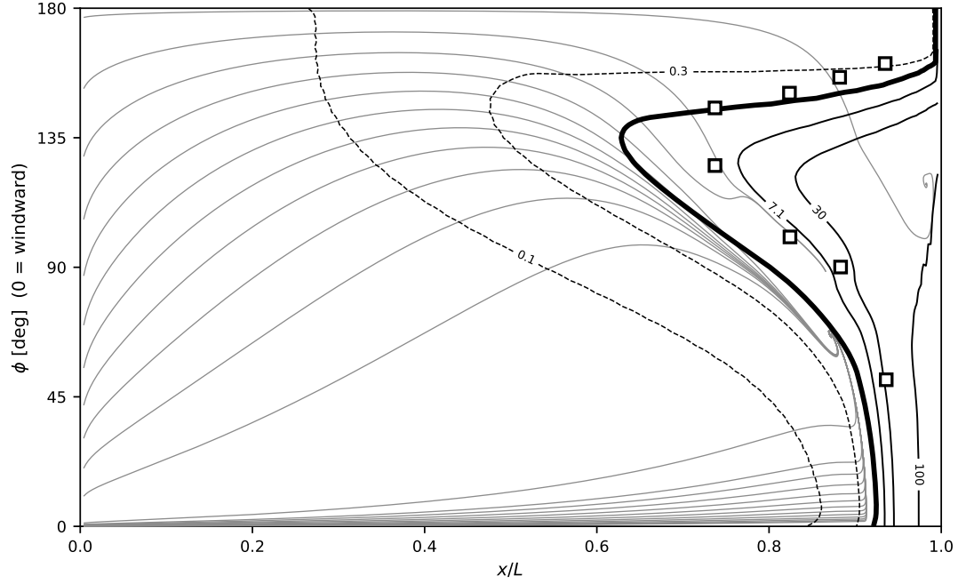
Figure 25: Surface at the measured-seed condition, unrolled into (x/L, \phi) , \phi = 0 windward; line art. Grey skin-friction lines integrated from the wall shear vector itself – the oil-flow analogue, not the inviscid streamlines of Stock Figs. 14–17, and their convergence is the separation signature – under the \max_n \chi contour family (sub-unity dashed, \chi = 1 heavy, \chi = c_{v1} and above solid, labeled), \max_n \chi taken on a wall-normal segment shot from each surface point. White-filled squares: measured DFVLR transition. \alpha = 5^\circ , Re_L = 1.52 \times 10^6 .
