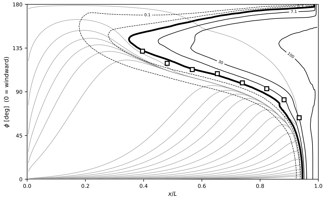
Figure 26: \alpha = 10^\circ , Re_L = 1.52 \times 10^6 .
