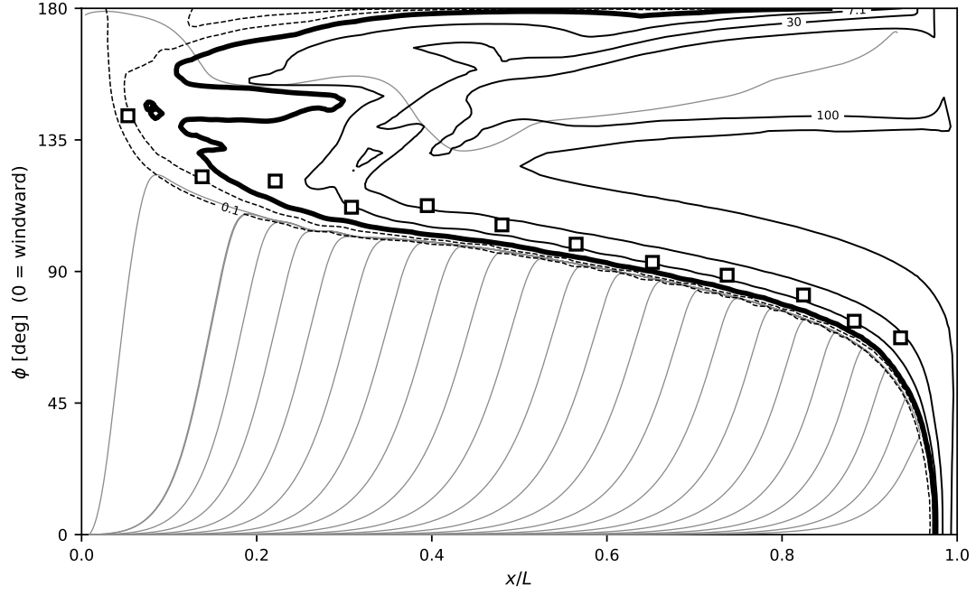
Figure 27: \alpha = 29.7^\circ , Re_L = 1.53 \times 10^6 ; the friction lines converge onto the open free-vortex-layer separation over most of the leeward half, and the twelve measured stations lie on that line rather than on a transition front.
