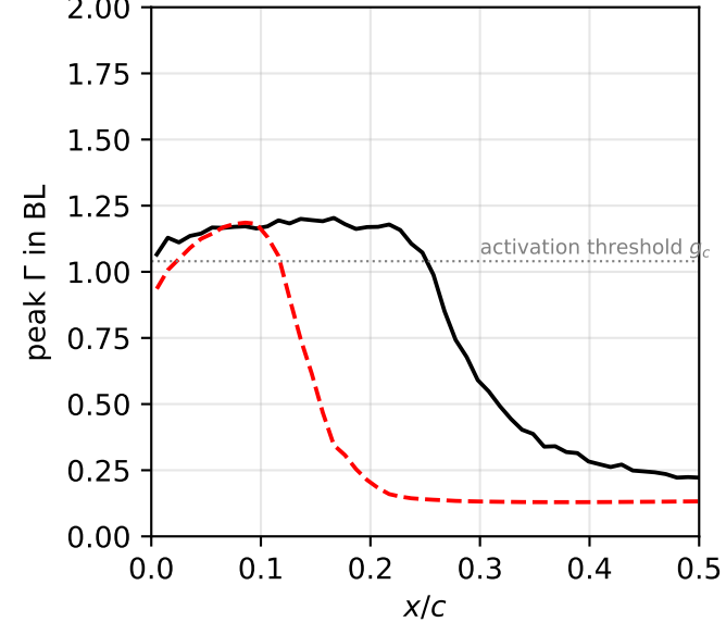
\Gamma peak vs. chord
