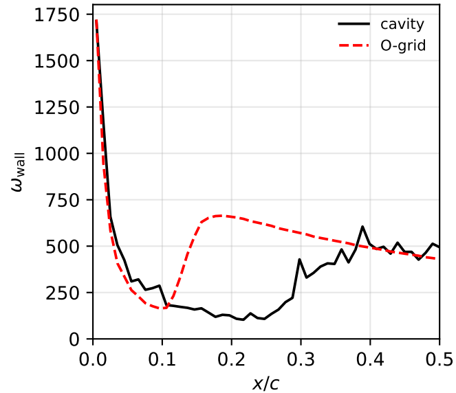
wall vorticity along chord
