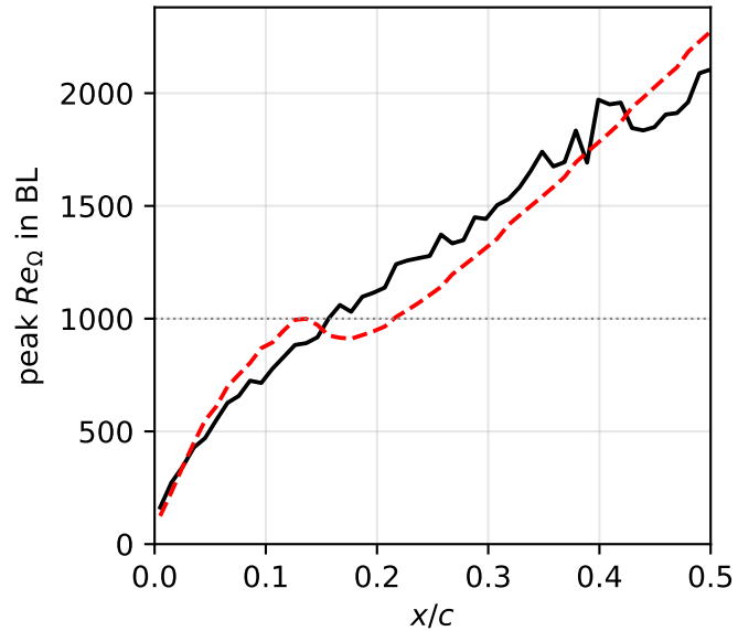
Re_{\Omega} peak vs. chord
