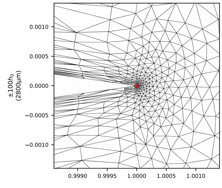
L0 ( h_0 = 14\mu\text{m} , r = 2.0 )
