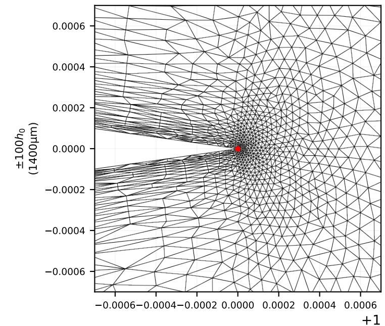
L1 ( h_0 = 7\mu\text{m} , r = 1.5 )
