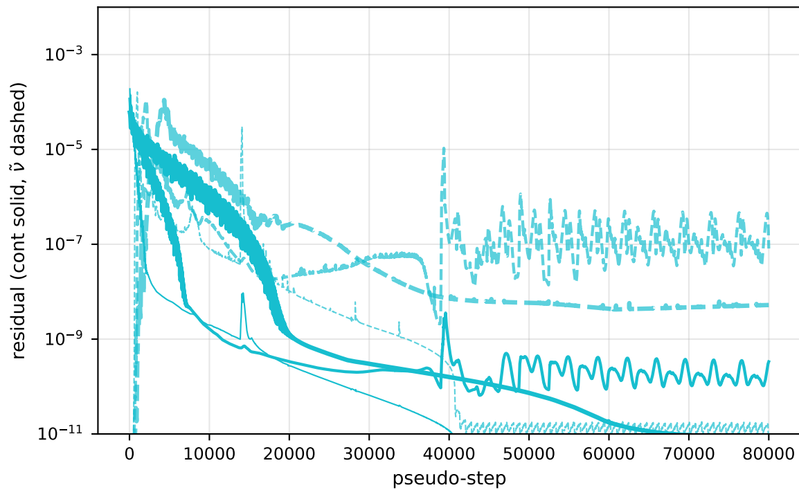
\alpha=15^\circ : residuals
