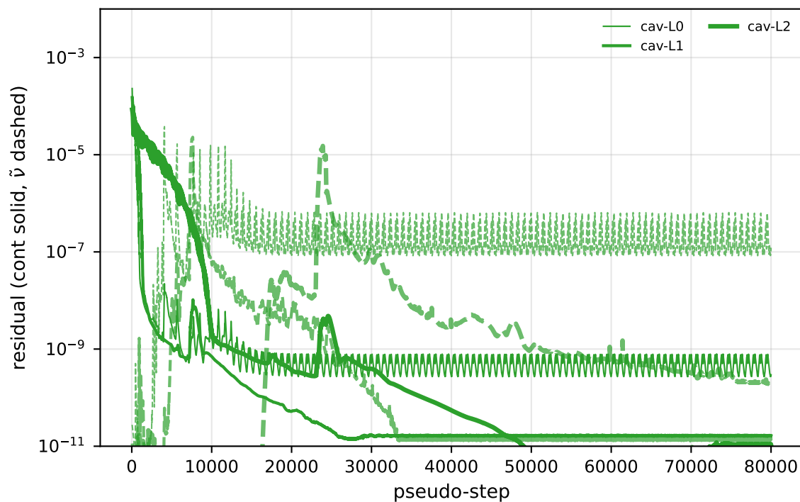
\alpha=4^\circ : residuals
