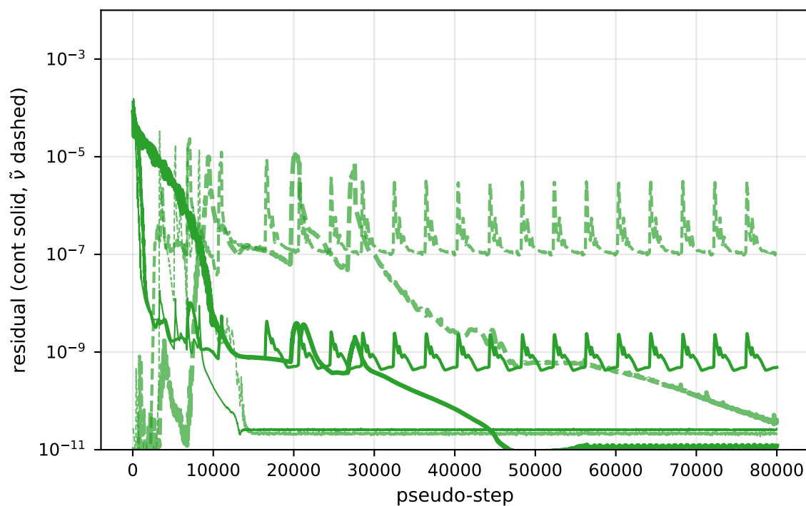
\alpha=4^\circ : residuals
