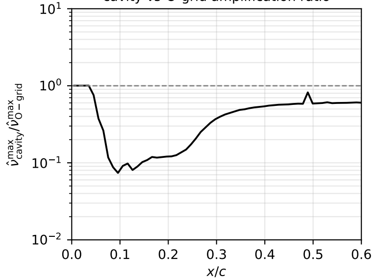
cavity-vs-O-grid amplification ratio
