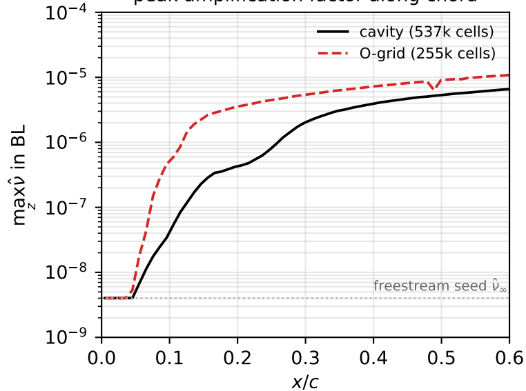
peak amplification factor along chord
