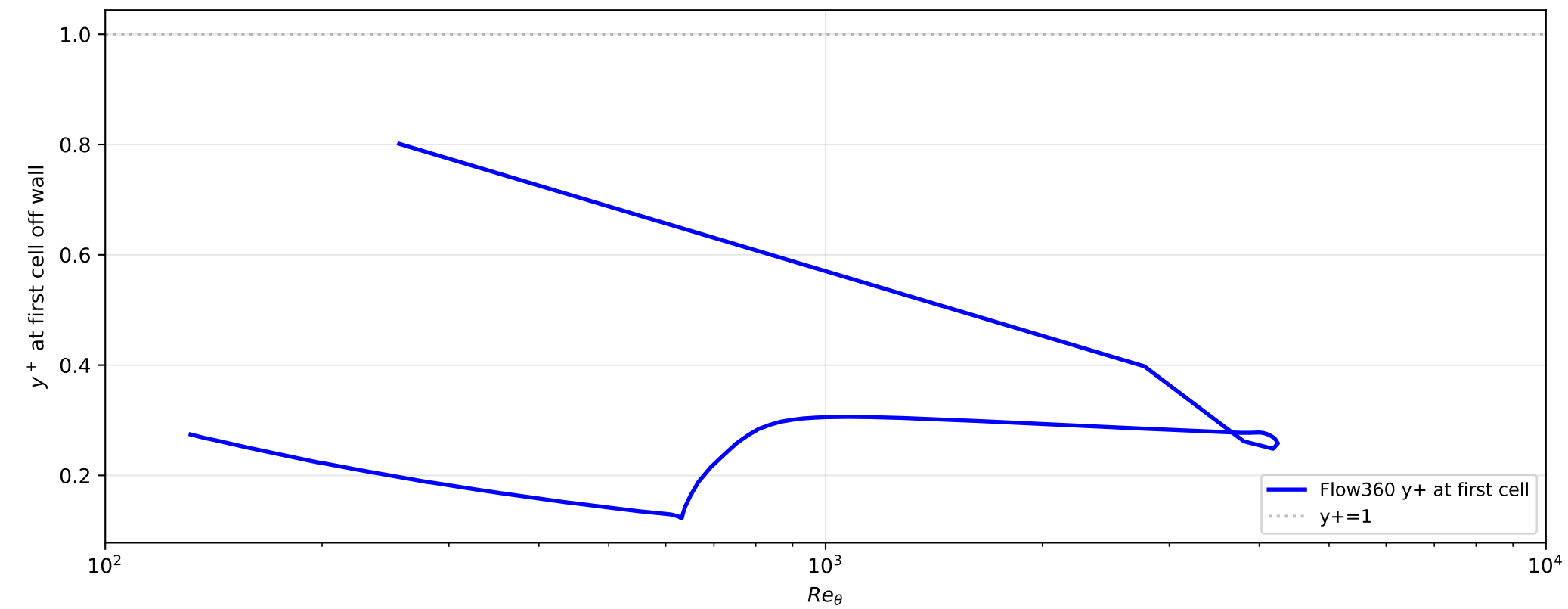
Wall resolution in Flow360
