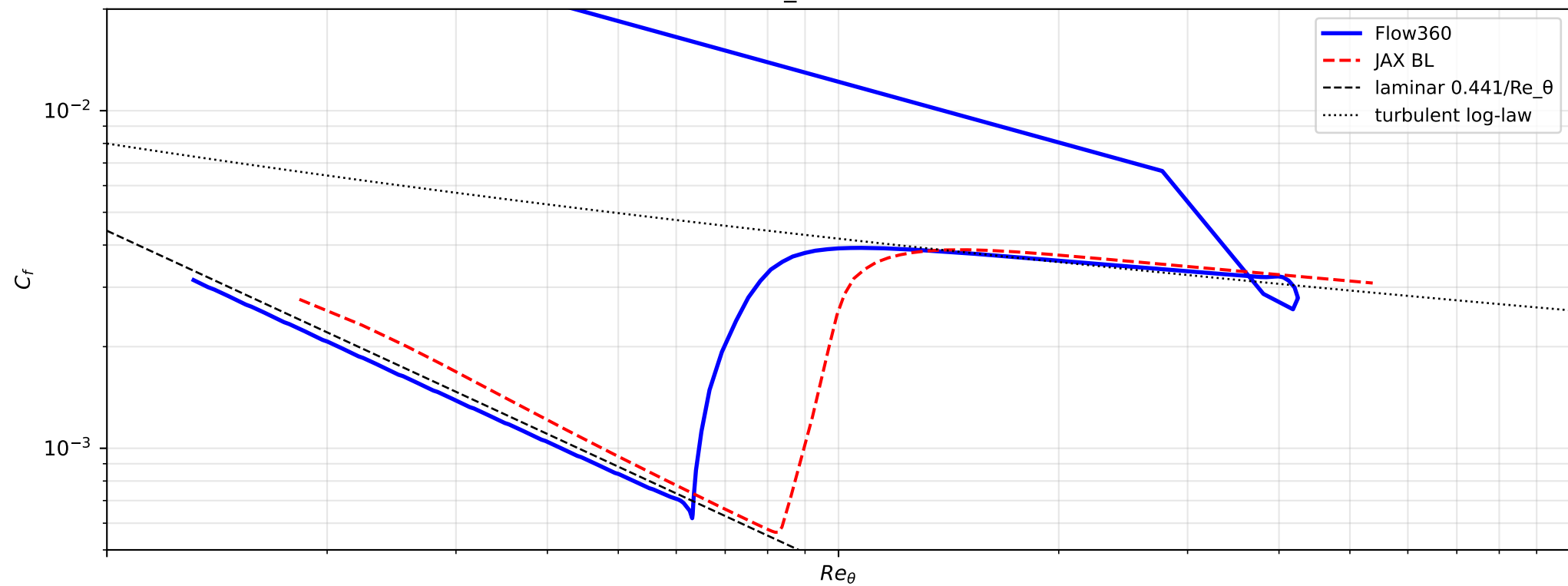
Wall resolution in Flow360
