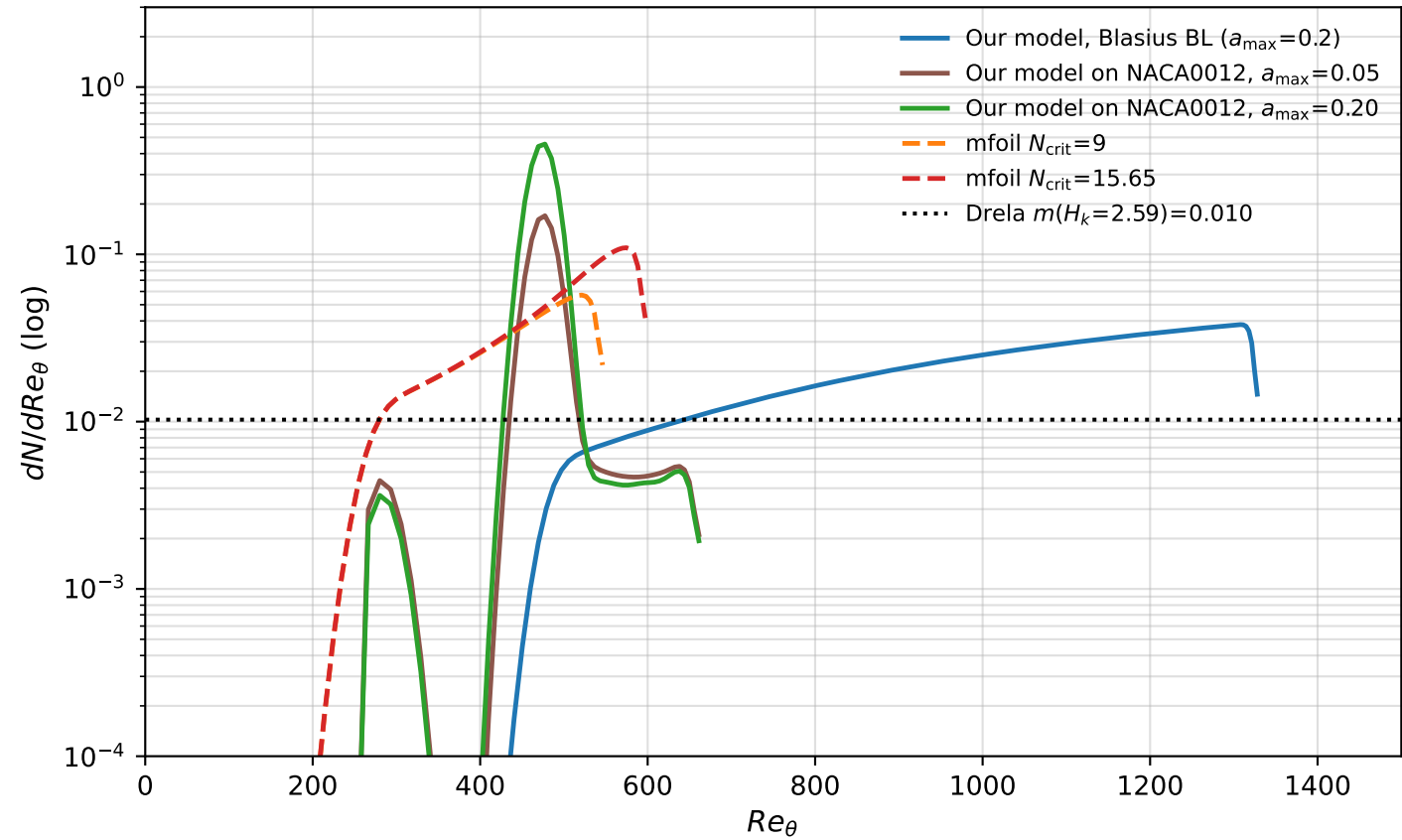
Amplification rate dN/dRe_\theta — what scales as what
