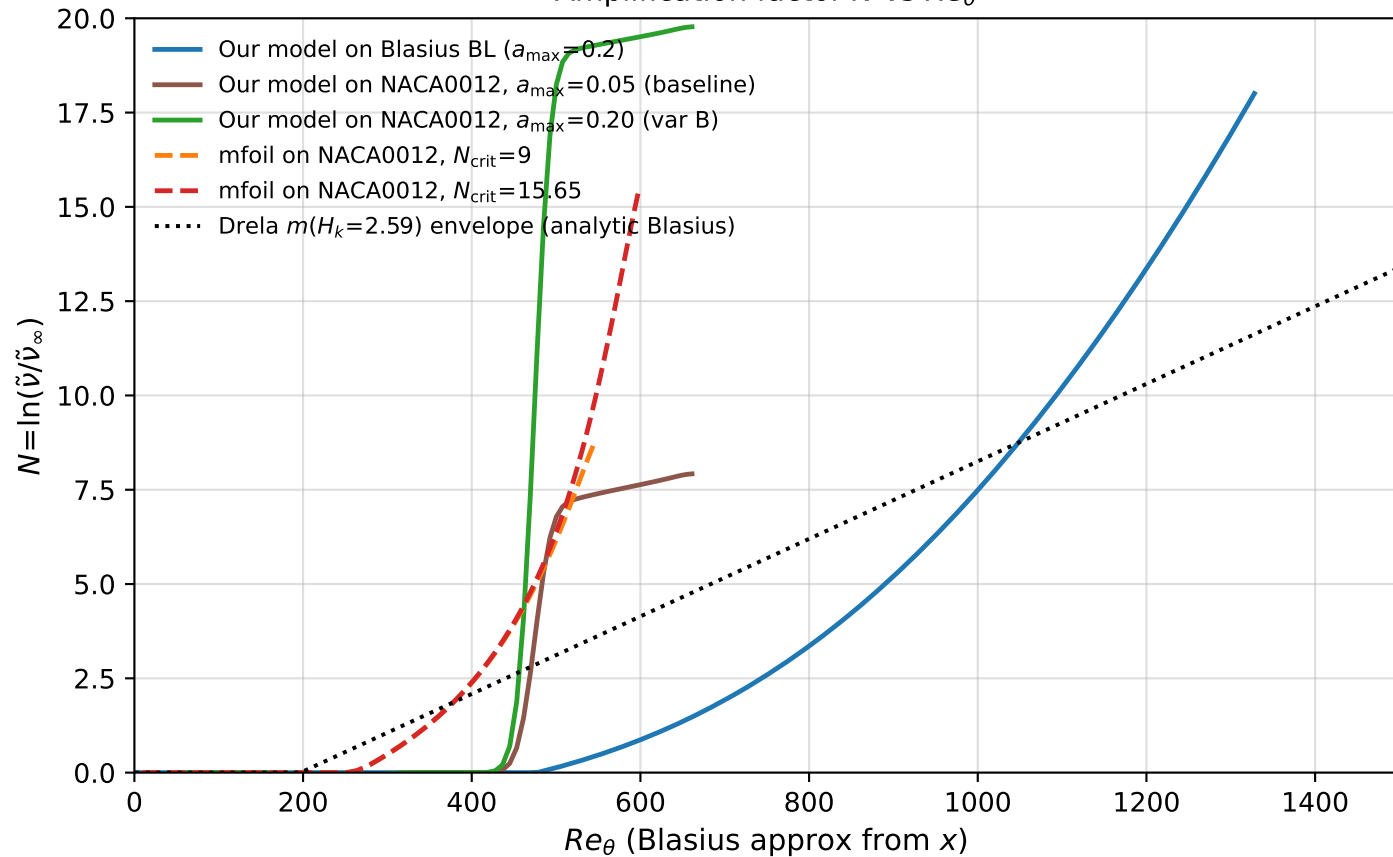
Amplification factor N vs Re_\theta
