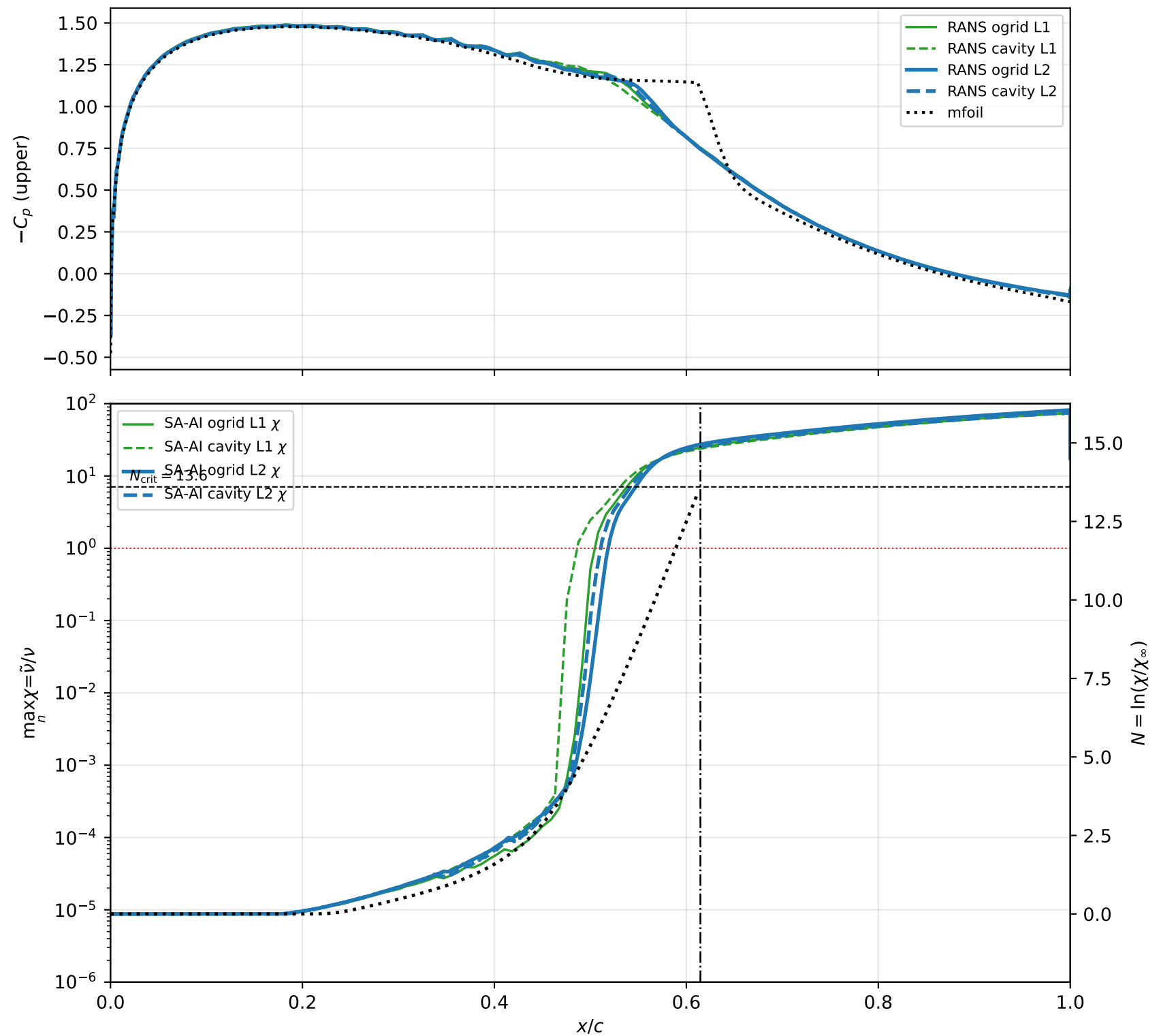
Daedalus section \eta = 0.305 , \alpha = 5^\circ , Re = 5e + 05 , c_l = 1.18 : SA-AI amplification vs mfoil e^N
