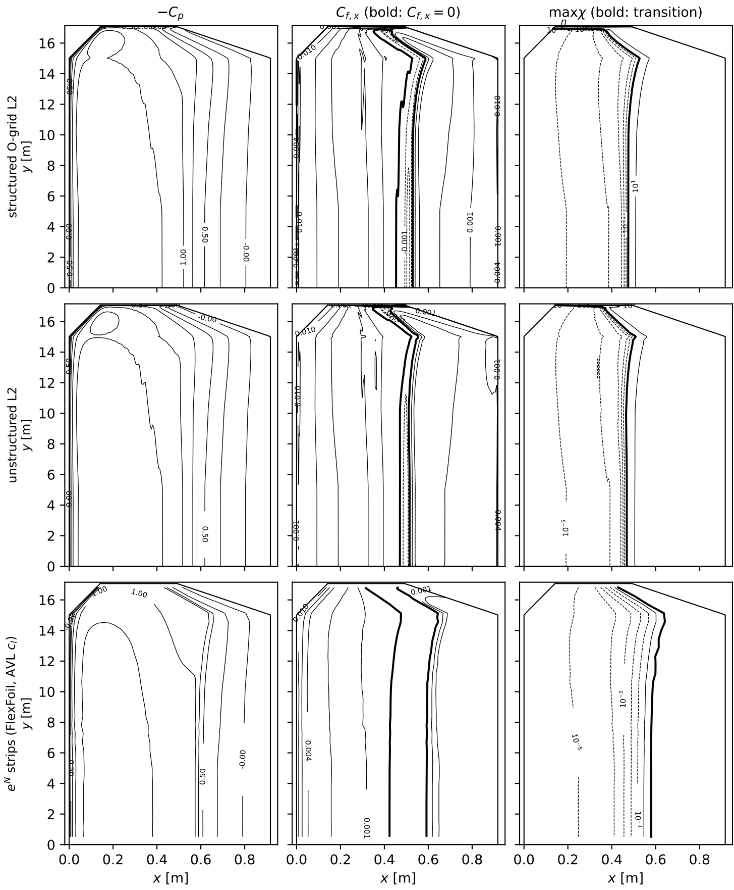
Daedalus wing, upper surface, \alpha = 5^\circ
