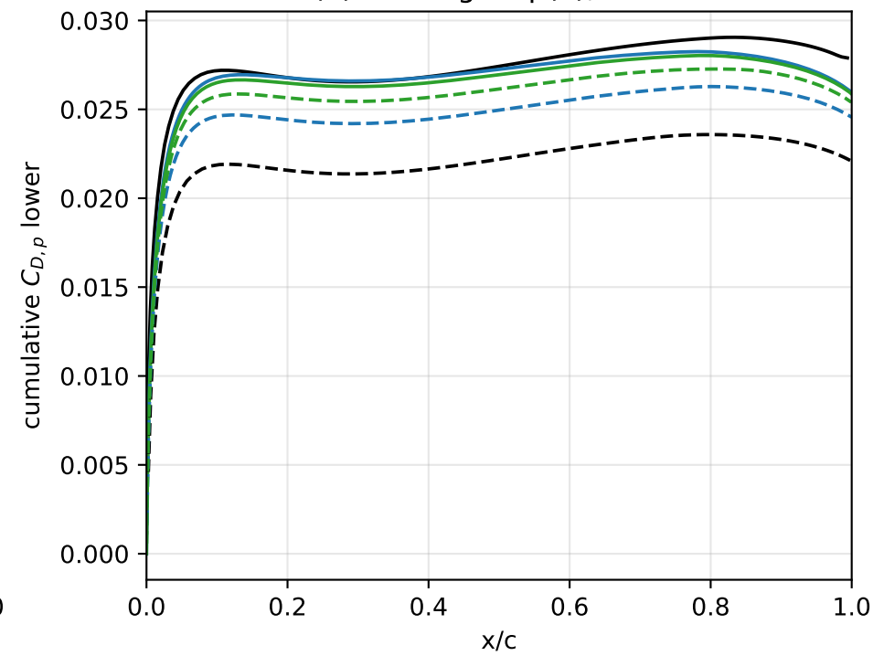
(e) running CD_p(x) , lower
