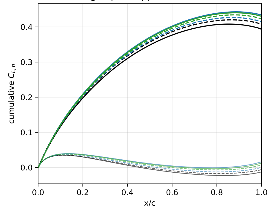
(f) running CL_p(x) , upper(solid)+lower(faint)
