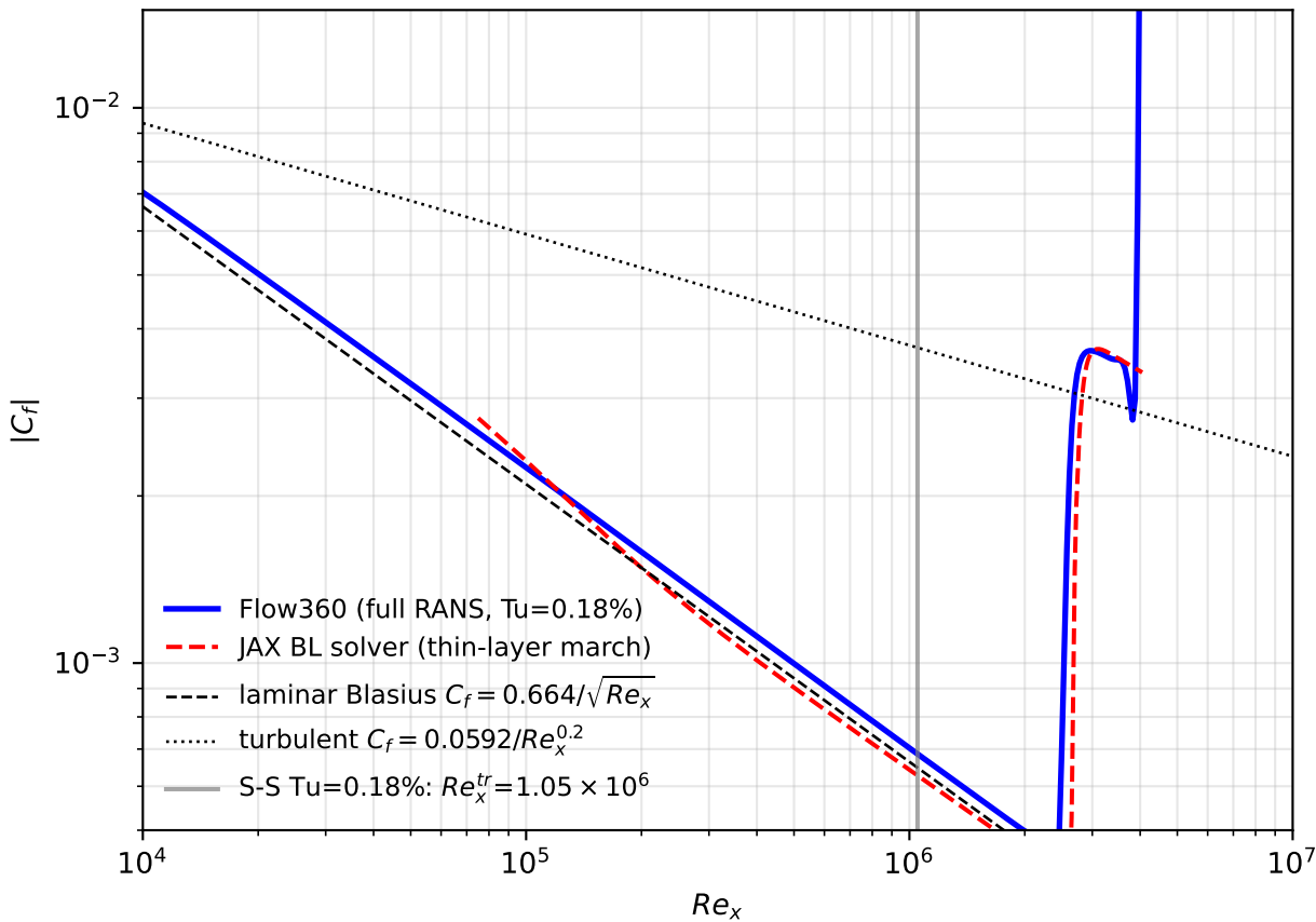
Flat plate at Tu=0.18\% : Flow360 vs JAX BL solver vs S-S
