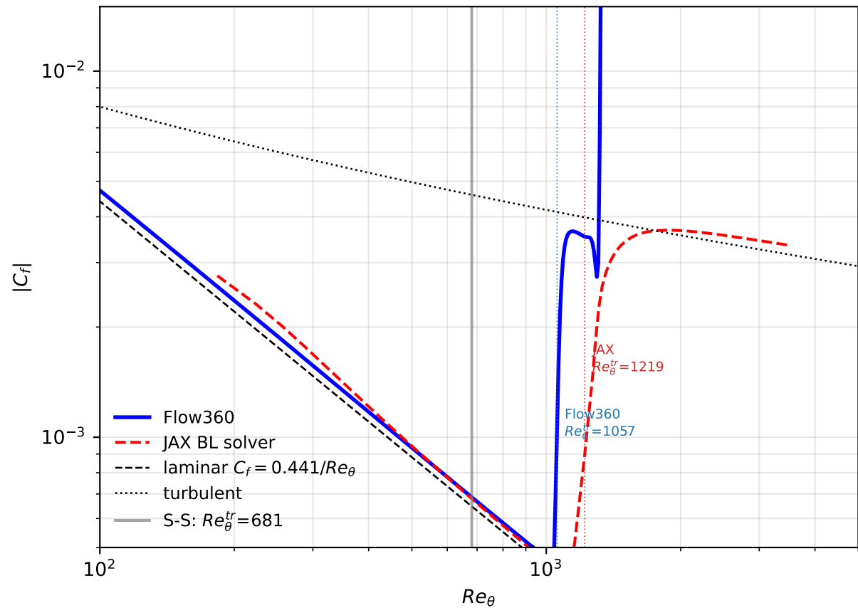
Same data on Re_\theta axis
