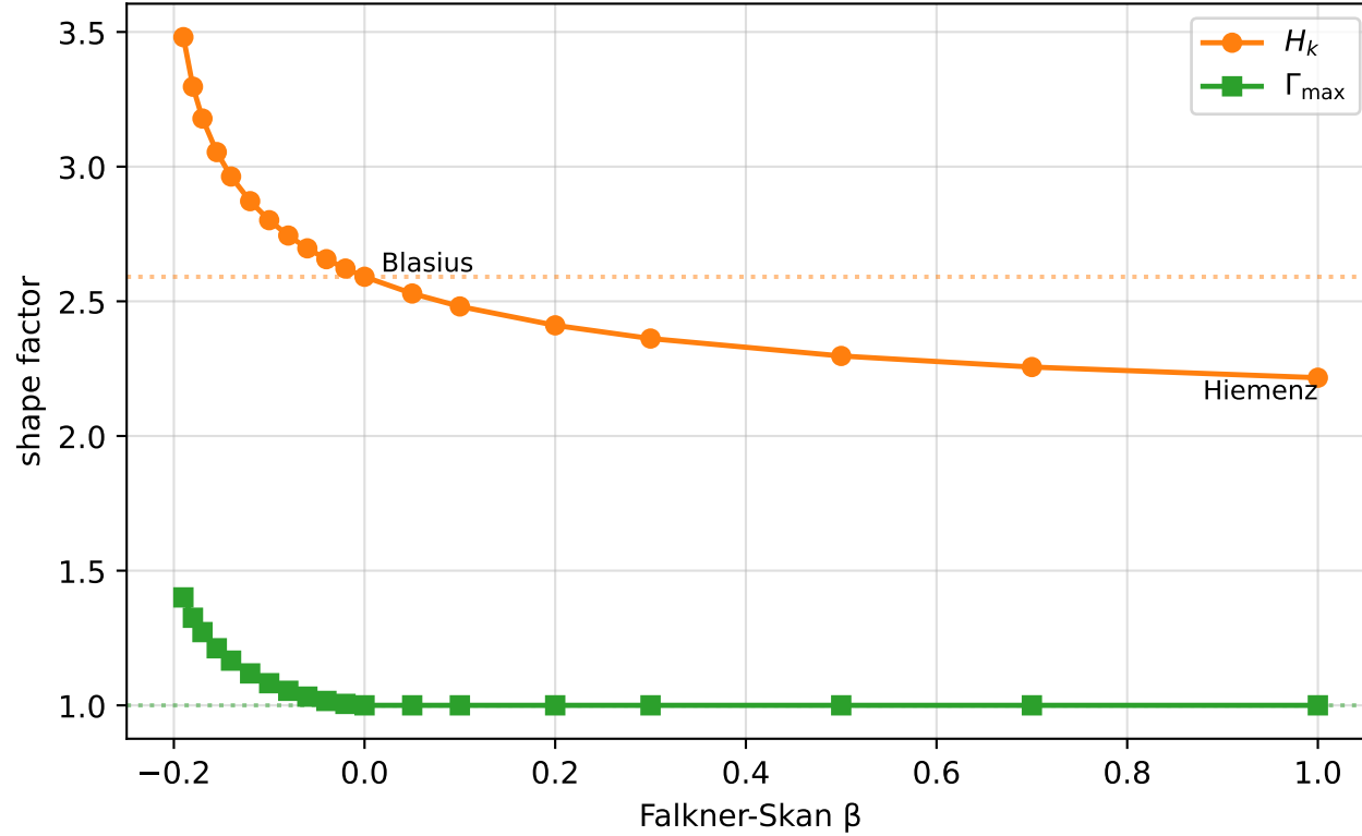
Falkner-Skan sweep: H_k(\beta) and \Gamma_{\max}(\beta)
