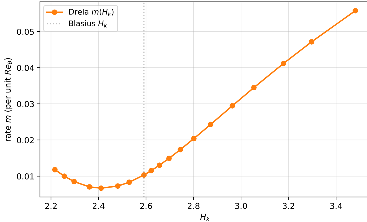
Drela's m(H_k) — the target rate curve
