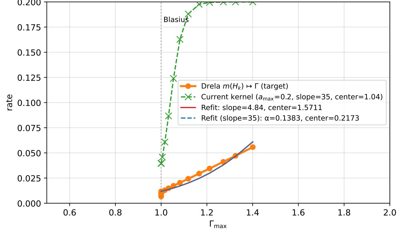
How sensitive should a(\Gamma) be? Match to Drela m(H_k) on FS
