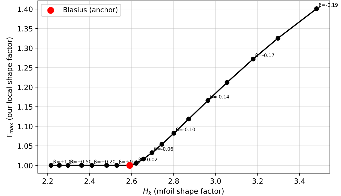
Mapping: \Gamma_{\max}(H_k) along FS family
