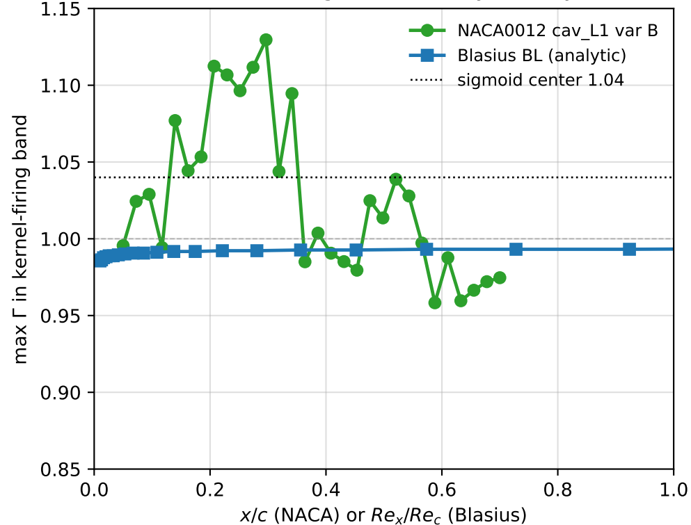
\Gamma_{\max}(x) along BL — the asymmetry
