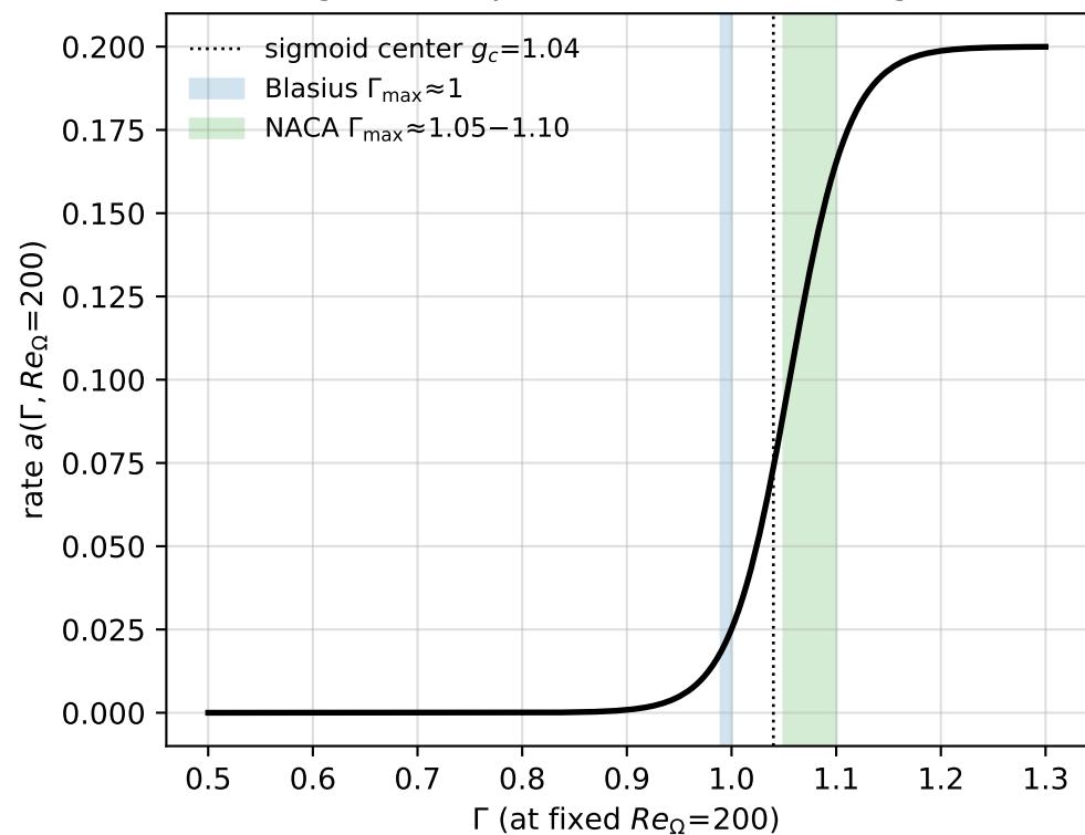
Sigmoid response — small \Delta\Gamma \rightarrow big \Delta a
