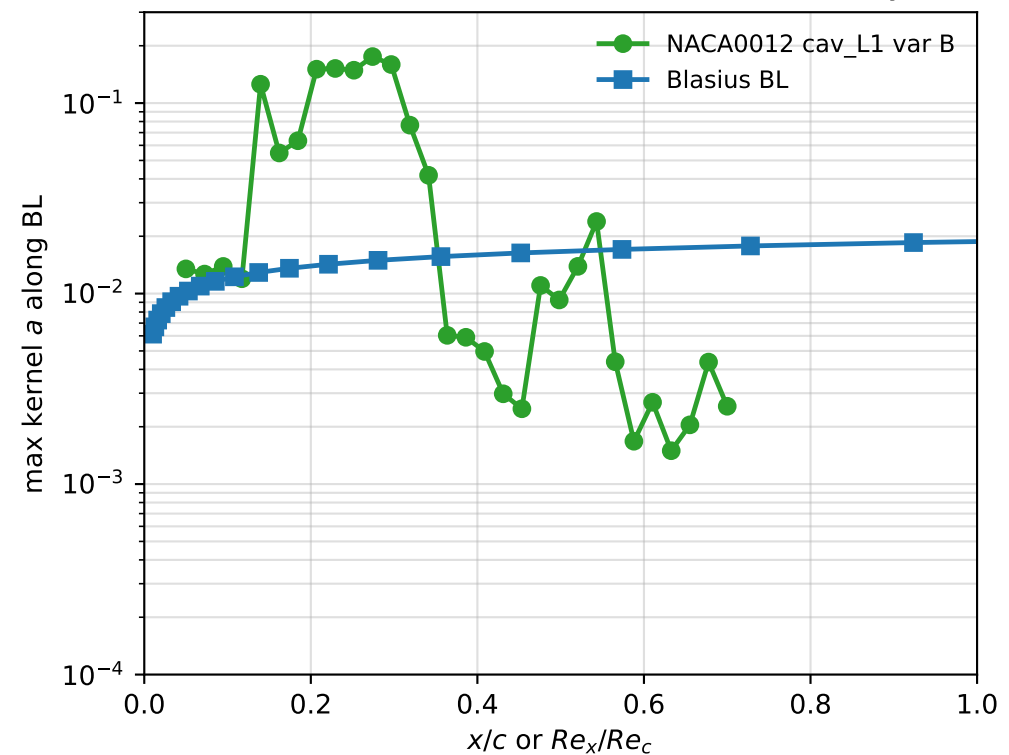
Kernel saturation: NACA fires a \rightarrow a_{\max} , Blasius stays small
