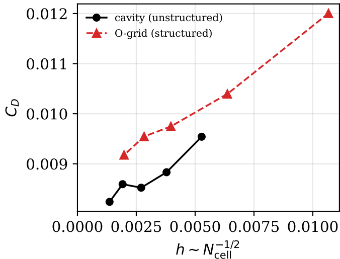
drag vs.\ mesh size, \alpha = 4^\circ
