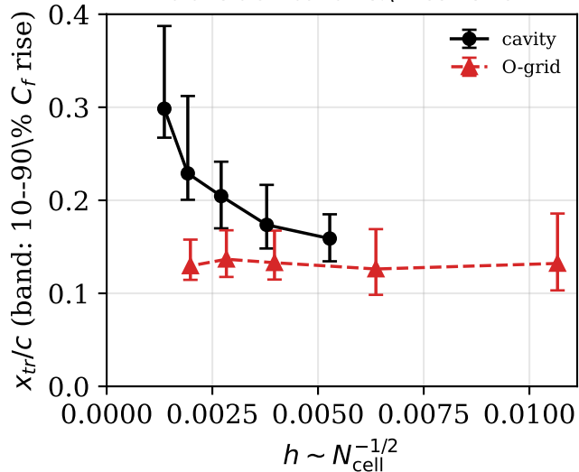
transition band vs.\ mesh size
