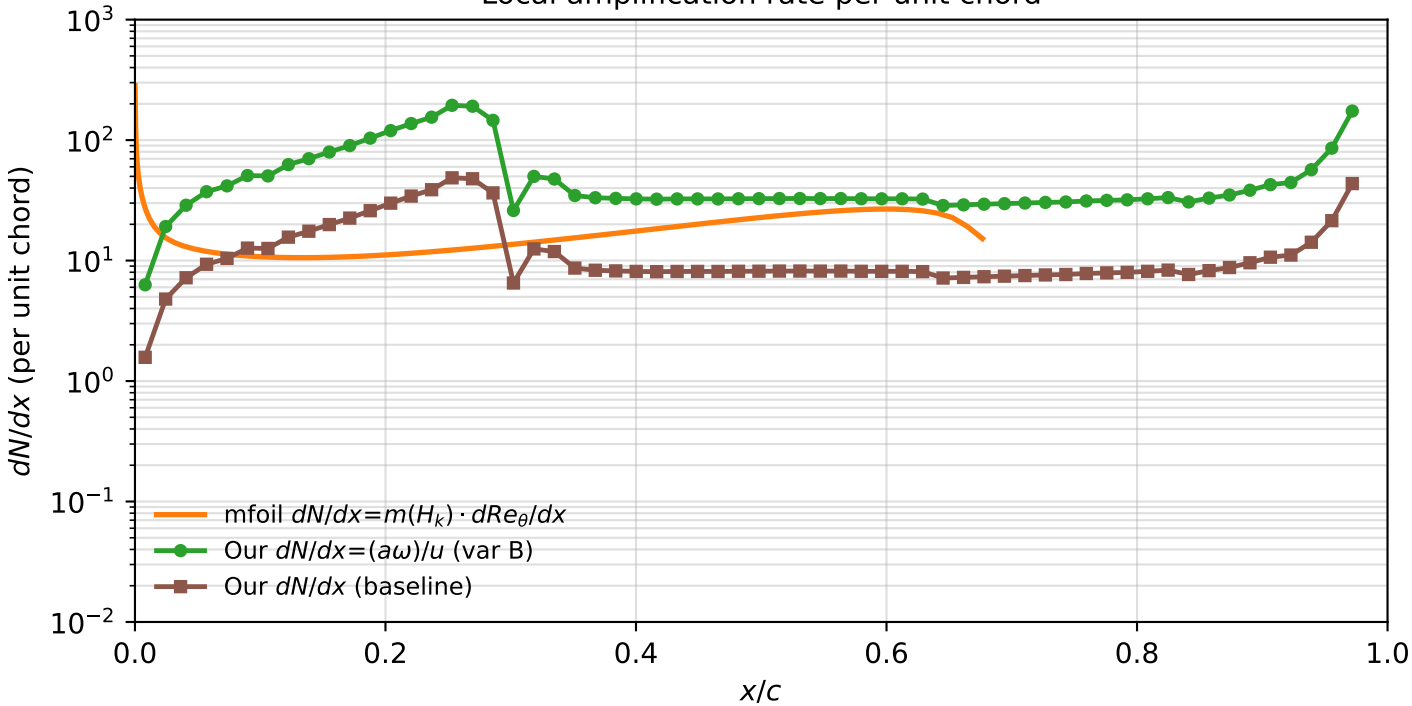
Local amplification rate per unit chord
