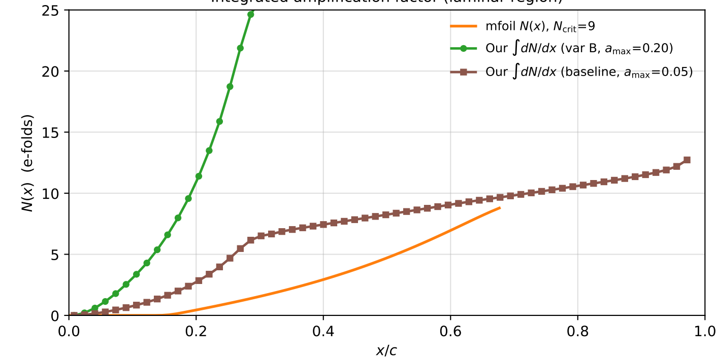
Integrated amplification factor (laminar region)
