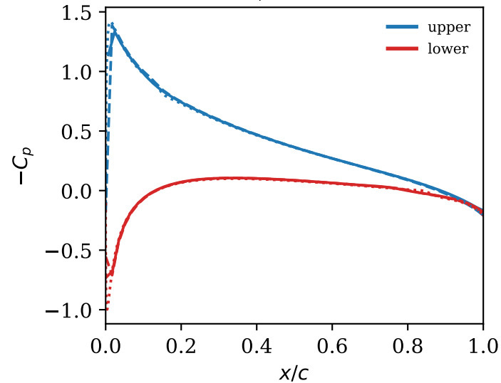
C_p, \alpha = 4^\circ
